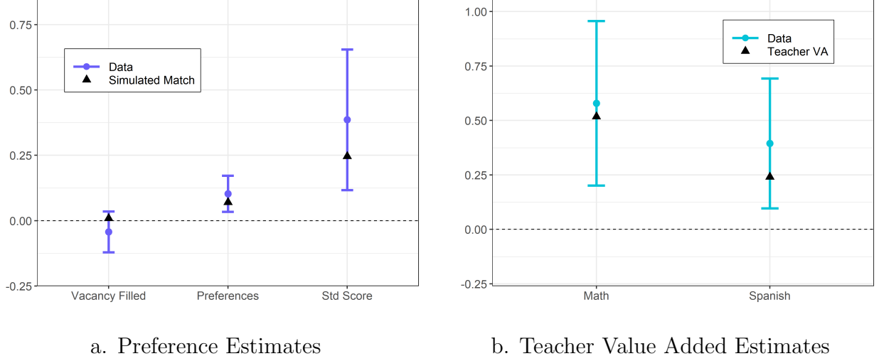
Figure 7: Model Validation
