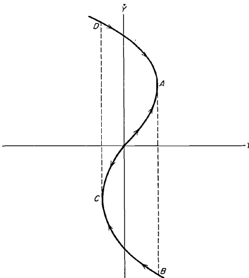
FIGURE 2 Phase Map of \psi
