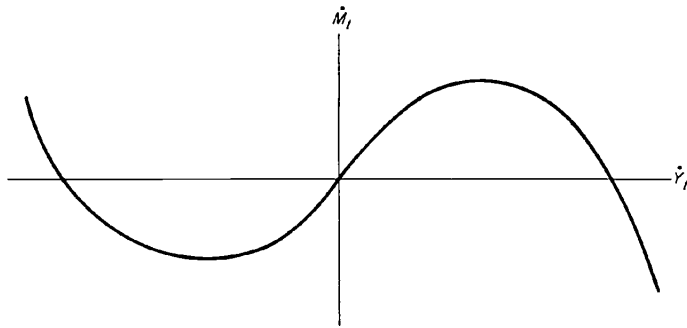
FIGURE 1 The \Omega Function
