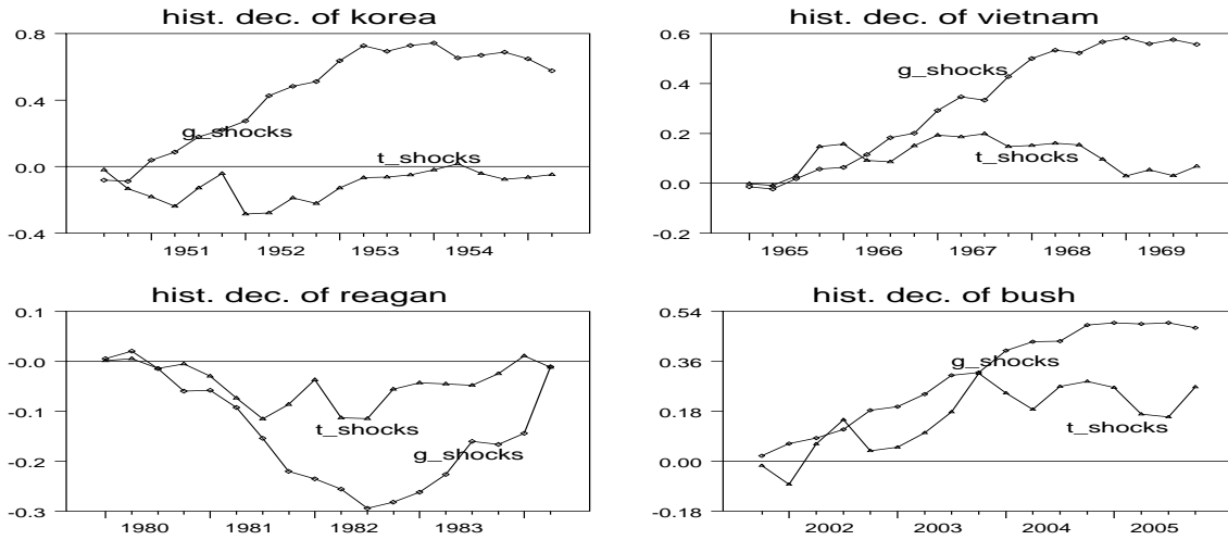
Figure 4: Historical decomposition of consumption, 1947:1-2005:4
