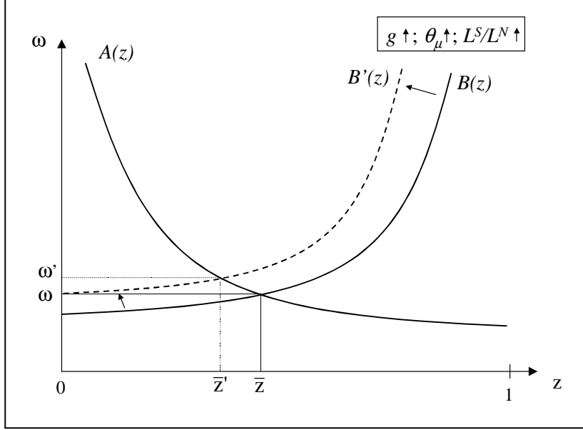
Figure 3: General Equilibrium
