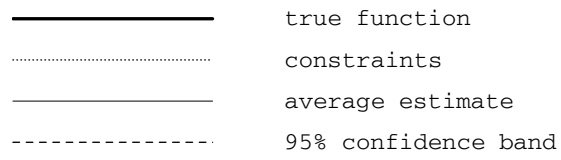
Figure 2: Locally Linear Estimator
