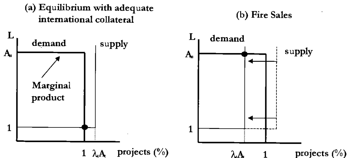
Figure 2: Fire Sales
