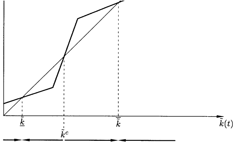
Fig. 7: Multiple locally stable steady states Either of the two possible limit points \tilde{k} or \underline{k} obtains, depending on \tilde{k}(0) \geq \tilde{k}^c . The dark kinked line describes \tilde{k}(t+1) as a function of \tilde{k}(t) in the Galor-Zeira model, as applied in Quah [92] to study economies confronting imperfect capital markets. If a cross section of economies had randomly distributed initial conditions \tilde{k}(0) , then over time the cross-section distribution of \tilde{k} 's (and thus of \tilde{y} 's) will tend towards a clustering around \underline{k} and \tilde{k} .
