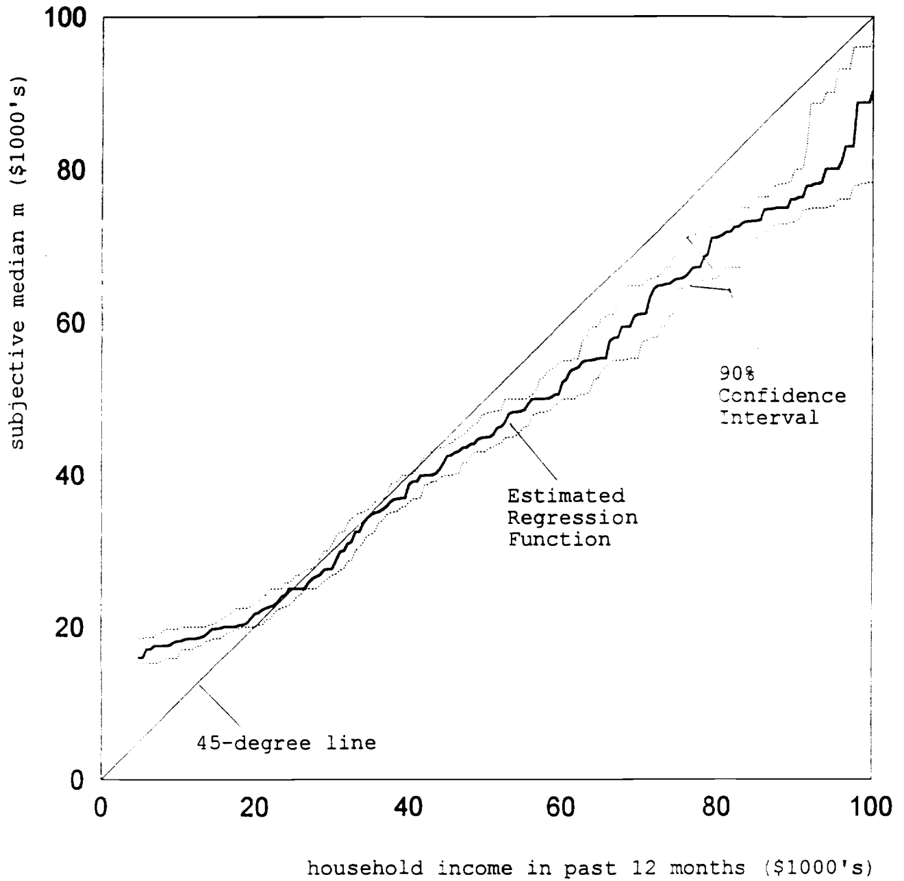
Figure 1: Best Prediction of Expectations Conditional on Realizations \text{Med}(m|y)
