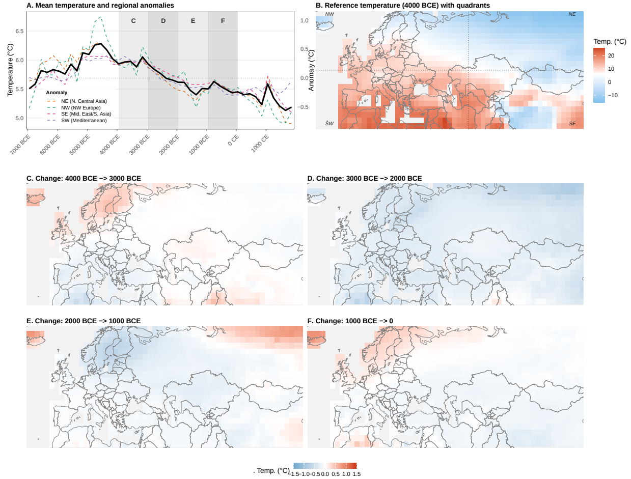
Figure A3: Paleoclimate Variation: Temperature over Time and Space
