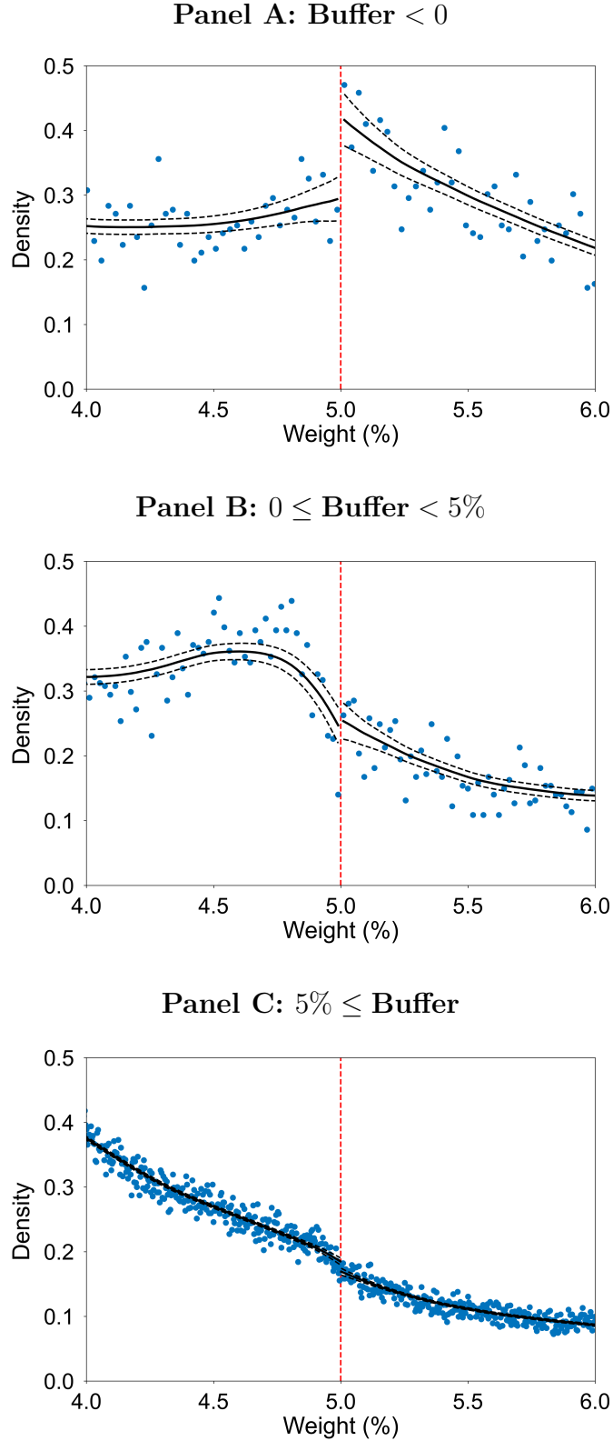
Figure 7. Bunching in funds' portfolio weights. This figure plots McCrory (2008) density estimates for 2019–2024 fund-stock-quarter observations. Circles denote histogram bins, solid lines show smooth densities, and dashed lines represent 95% confidence intervals. Panels A, B, and C correspond to funds with \text{Buffer} < 0 , 0 \leq \text{Buffer} < 5\% , and 5\% \leq \text{Buffer} , respectively.
