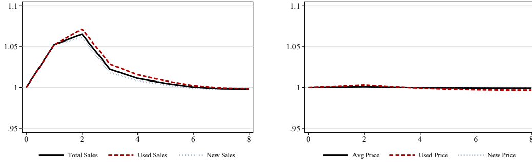
Panel B. Inelastic New Car Supply ( \varepsilon_s = 3.1 , 4 periods)
