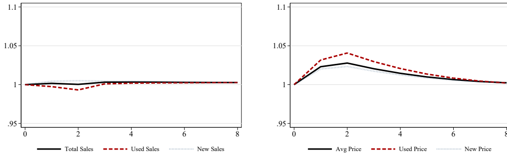
Panel D. Inelastic New Car Supply ( \varepsilon_s = 0.06 , permanent)
