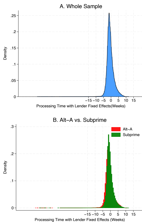
FIGURE B.1: Histogram of Processing Time Residuals Between 2002 and 2007
