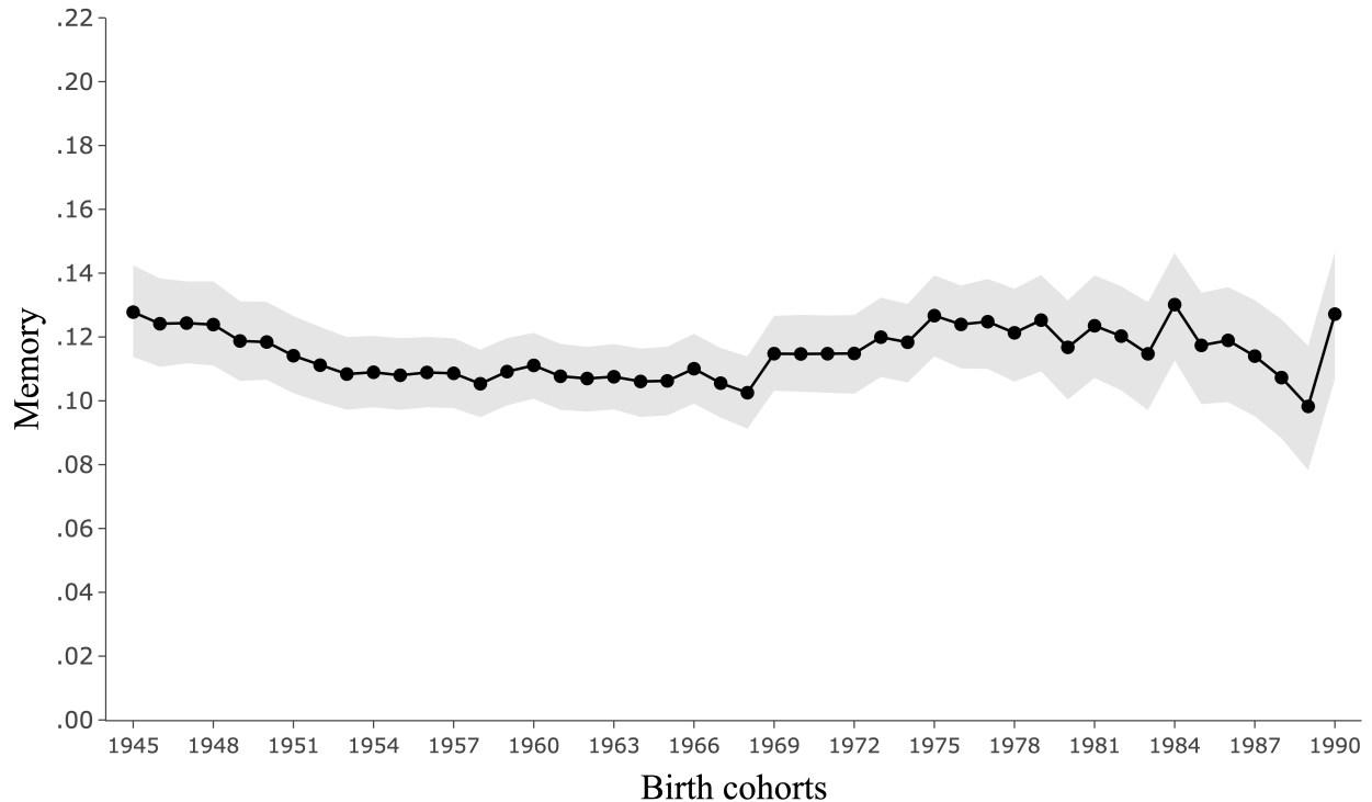
Figure 5: Aggregate intergenerational memory at generation t = 1 ( AIM_1 )
