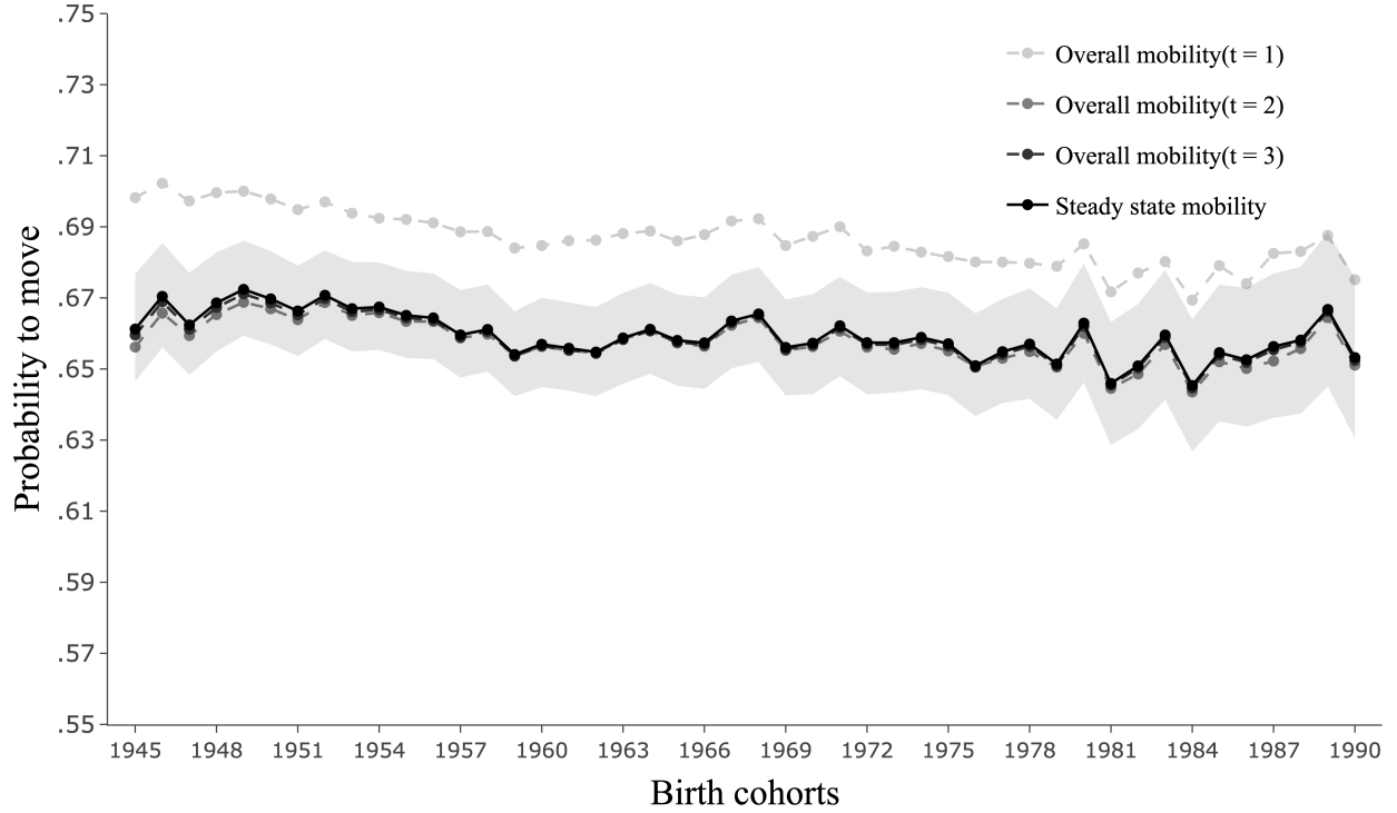
Figure 3: Overall mobility ( OM_t ) across synthetic generations
