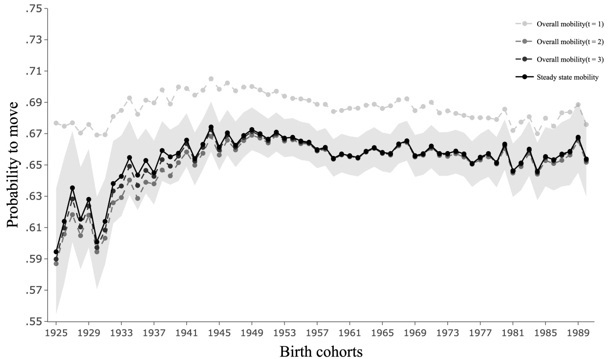
Figure H.2: Overall mobility ( OM_t ) across synthetic generations based on cohorts born between 1925 and 1985
