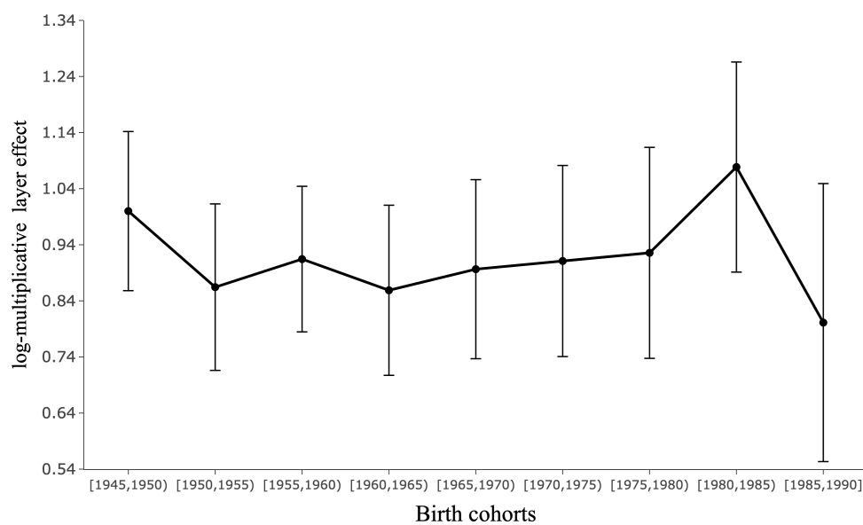
Figure F.4: Log-multiplicative layer effects based on White father-child pairs
