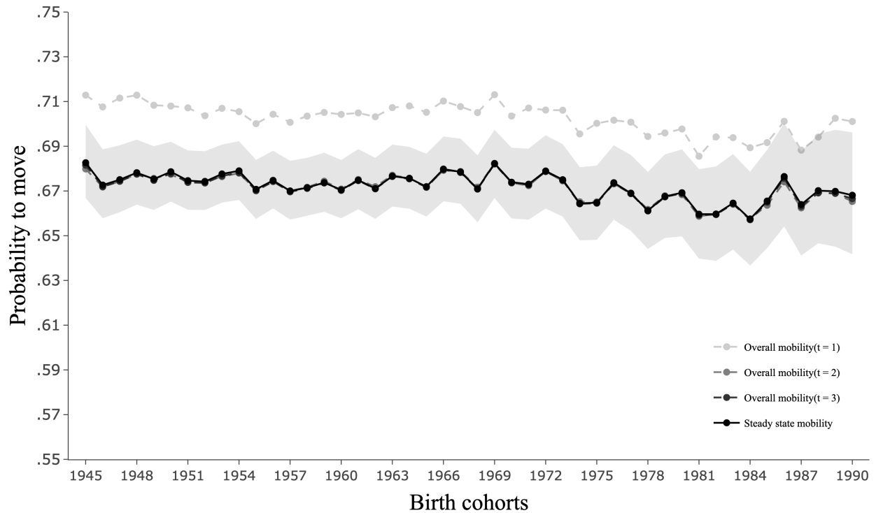
Figure F.2: Overall mobility ( OM_t ) across synthetic generations based on White father-child pairs
