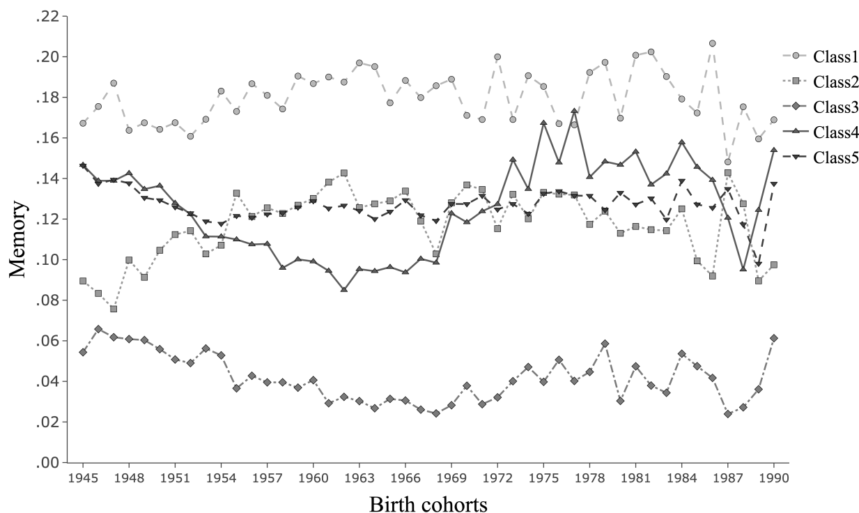
Figure 7: Intergenerational memory at generation t = 1 by origin class ( IM_{i,1} )
