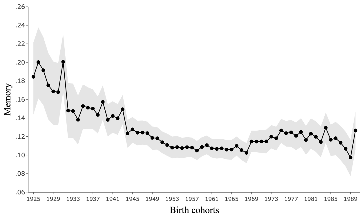
Figure H.3: Aggregate intergenerational memory at generation t = 1 ( AIM_1 ) based on cohorts born between 1925 and 1985
