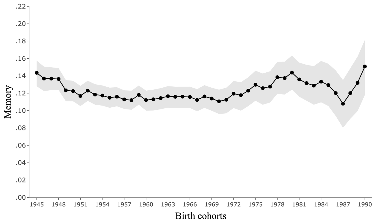
Figure A.7: Aggregate intergenerational memory at generation t = 1 ( AIM_1 ) computed from samples of respondents age 30-64
