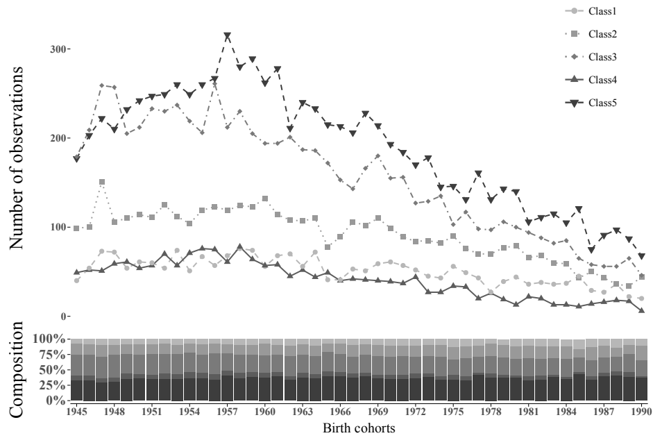
(A) Class destinations of children
