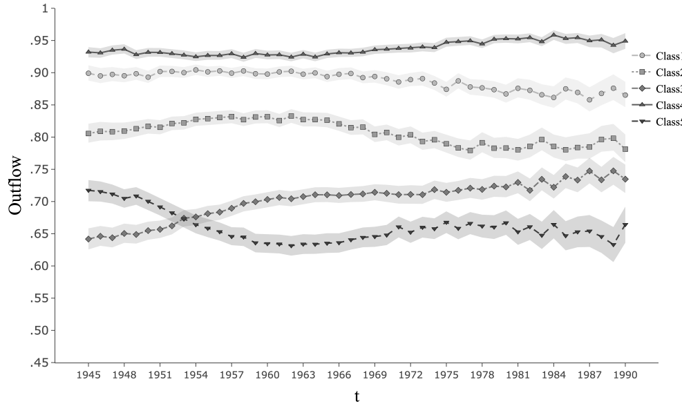
(B) Outflows at the steady state
