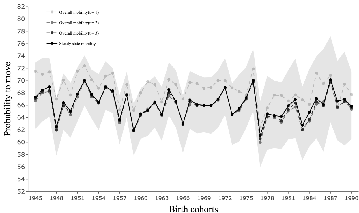
Figure G.8: Overall mobility ( OM_t ) across synthetic generations based on unsmoothed data
