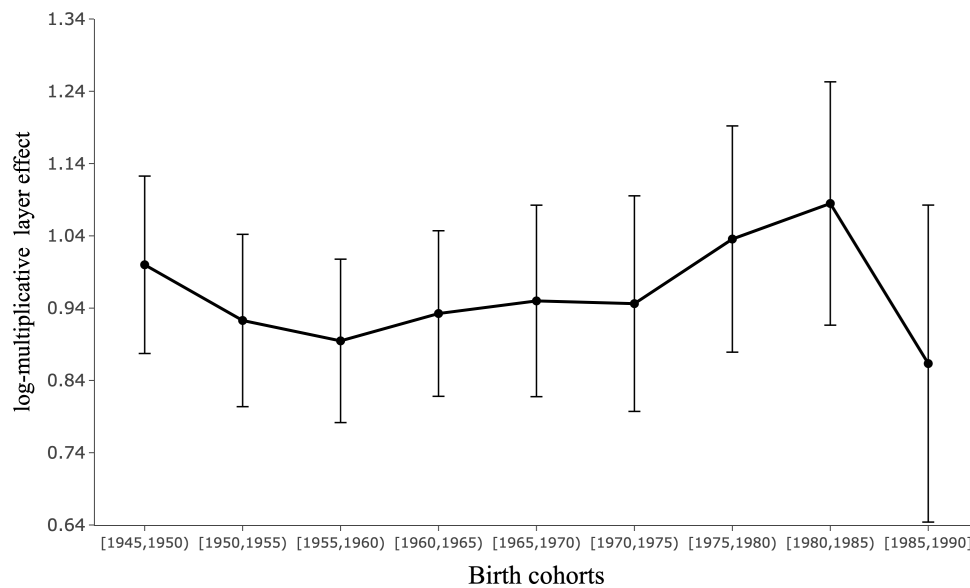
Figure A.8: Log-multiplicative layer effects computed from samples of respondents age 30-64
