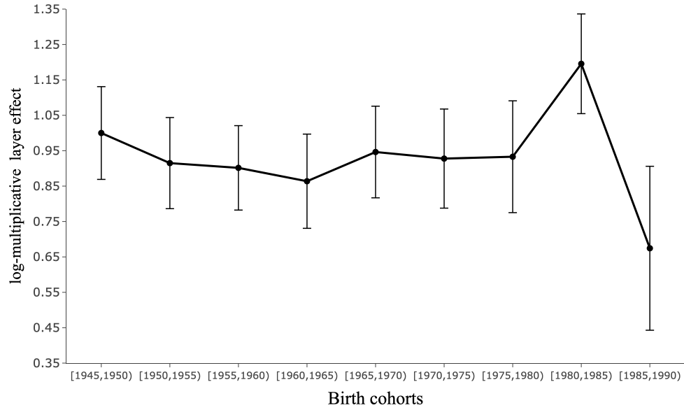
(A) Cohorts in 5-year bins
