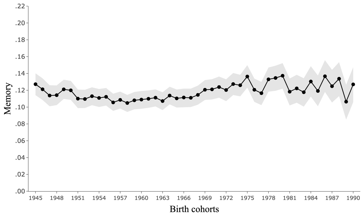
Figure B.7: Aggregate intergenerational memory at generation t = 1 ( AIM_1 ) based on the Morgan (2017) typology
