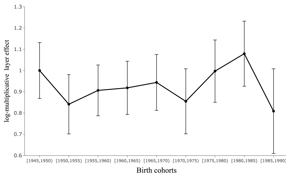
Figure B.12: Log-multiplicative layer effects excluding farmers
