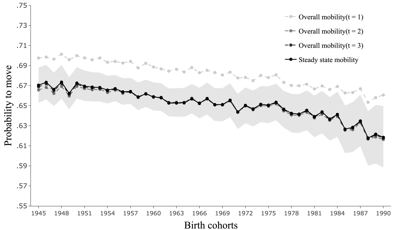
Figure C.2: Overall mobility ( OM_t ) across synthetic generations
