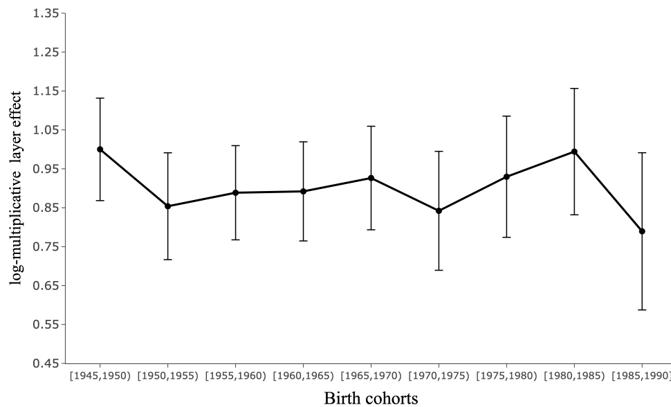
Figure B.16: Log-multiplicative layer effects based on Erikson and Goldthorpe (2010) typology
