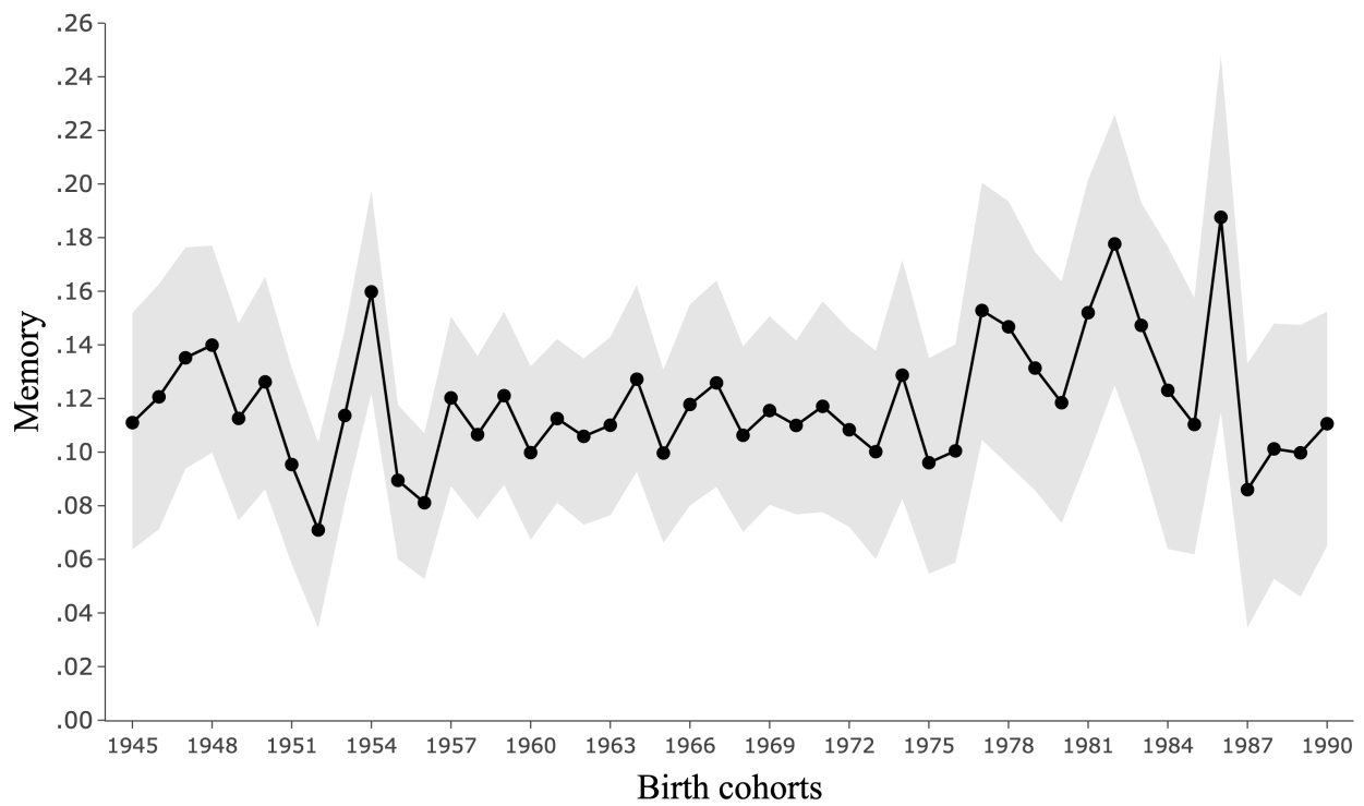
Figure G.9: Aggregate intergenerational memory at generation t = 1 ( AIM_1 ) based on unsmoothed data
