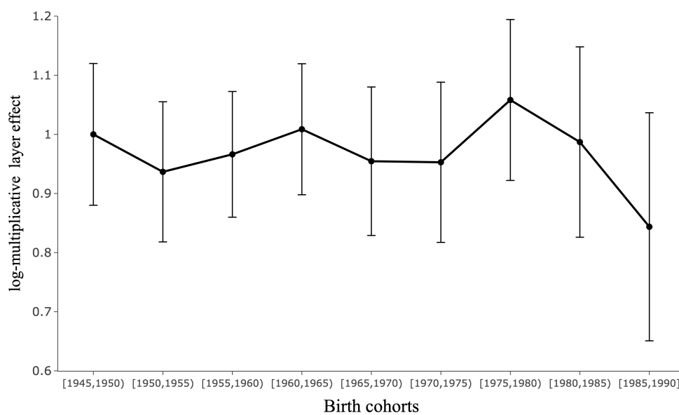
Figure B.8: Log-multiplicative layer effects based on the Morgan (2017) typology
