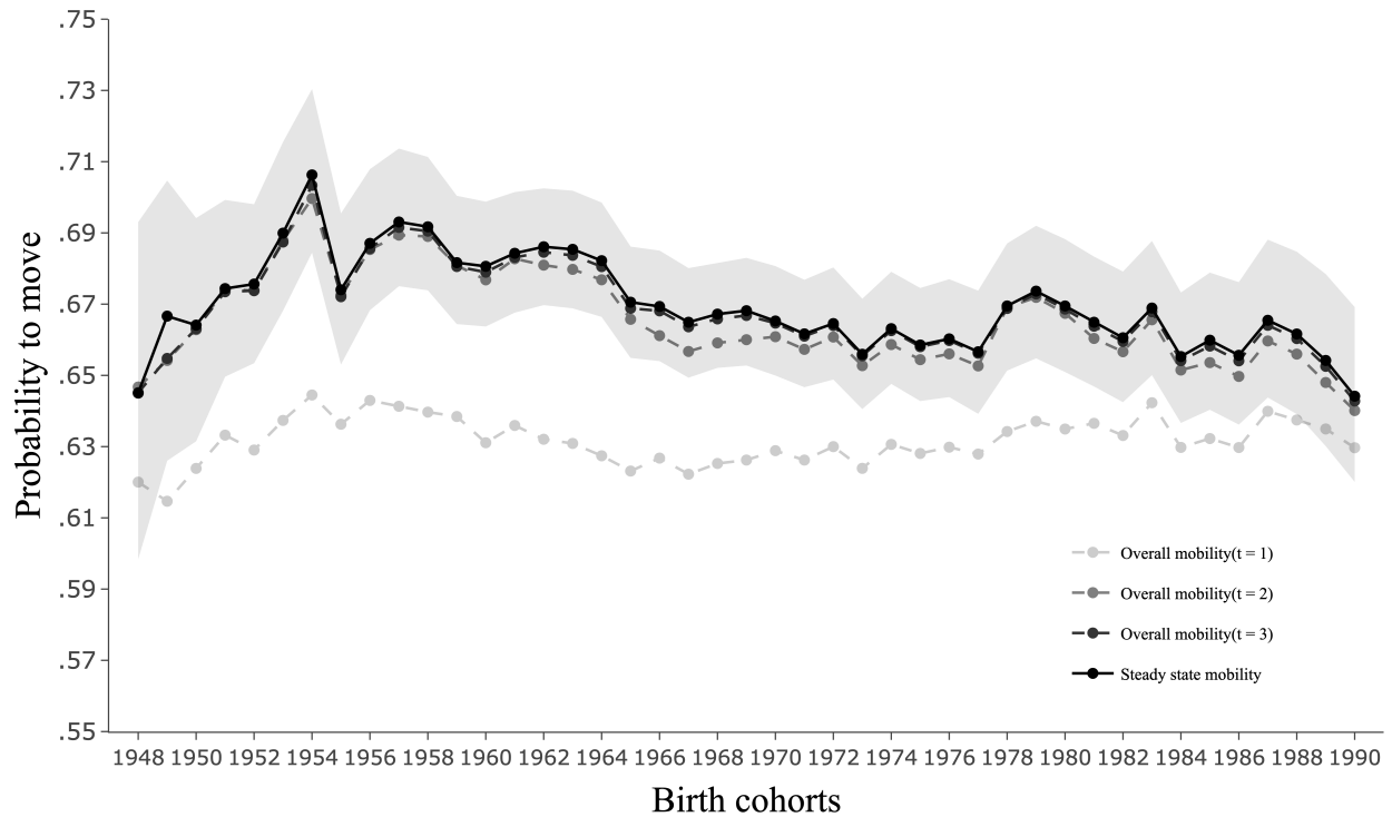
Figure E.10: Overall mobility ( OM_t ) across synthetic generations based on mother-child pairs
