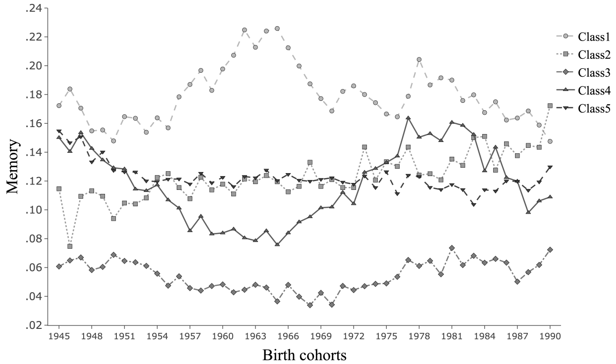
Figure C.5: Intergenerational memory at generation t = 1 by origin class ( IM_{i,1} )
