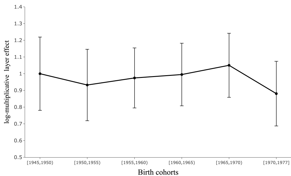
Figure E.4: Log-multiplicative layer effects based on father-daughter pairs
