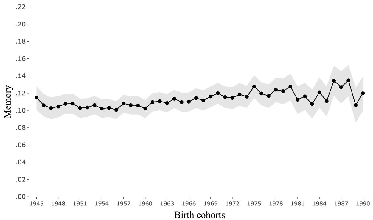
Figure B.3: Aggregate intergenerational memory at generation t = 1 ( AIM_1 ) based on the Pfeffer and Hertel (2015) typology
