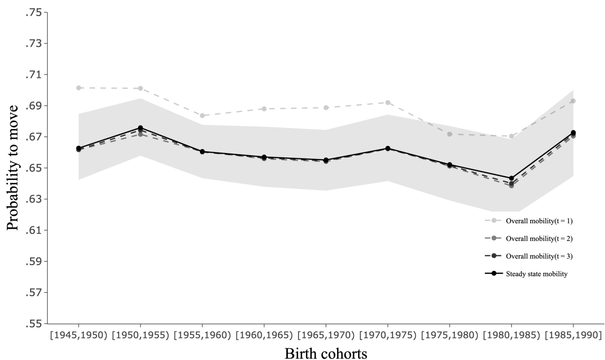
Figure G.5: Overall mobility ( OM_t ) across synthetic generations based on 5-year cohort bins
