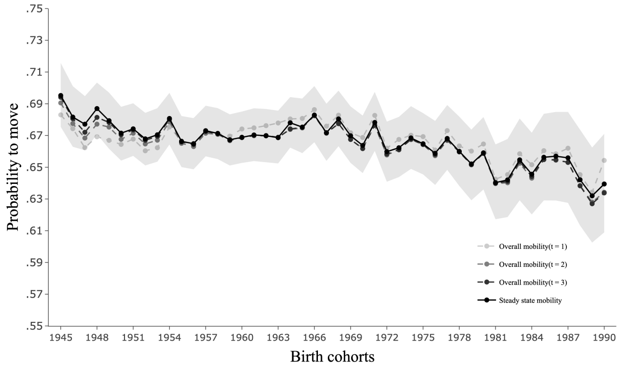
Figure E.6: Overall mobility ( OM_t ) across synthetic generations based on father-son pairs
