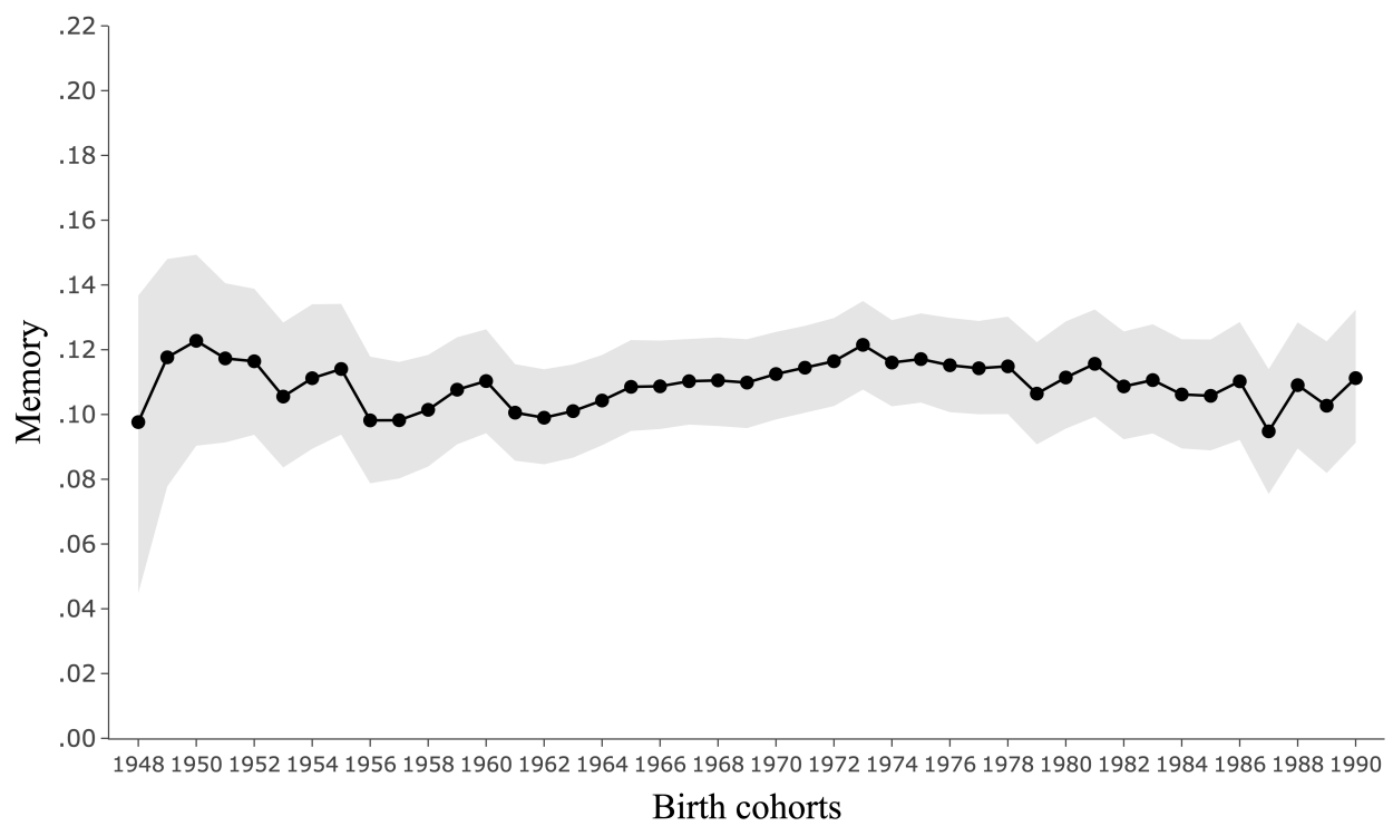
Figure E.11: Aggregate intergenerational memory at generation t = 1 ( AIM_1 ) based on mother-child pairs
