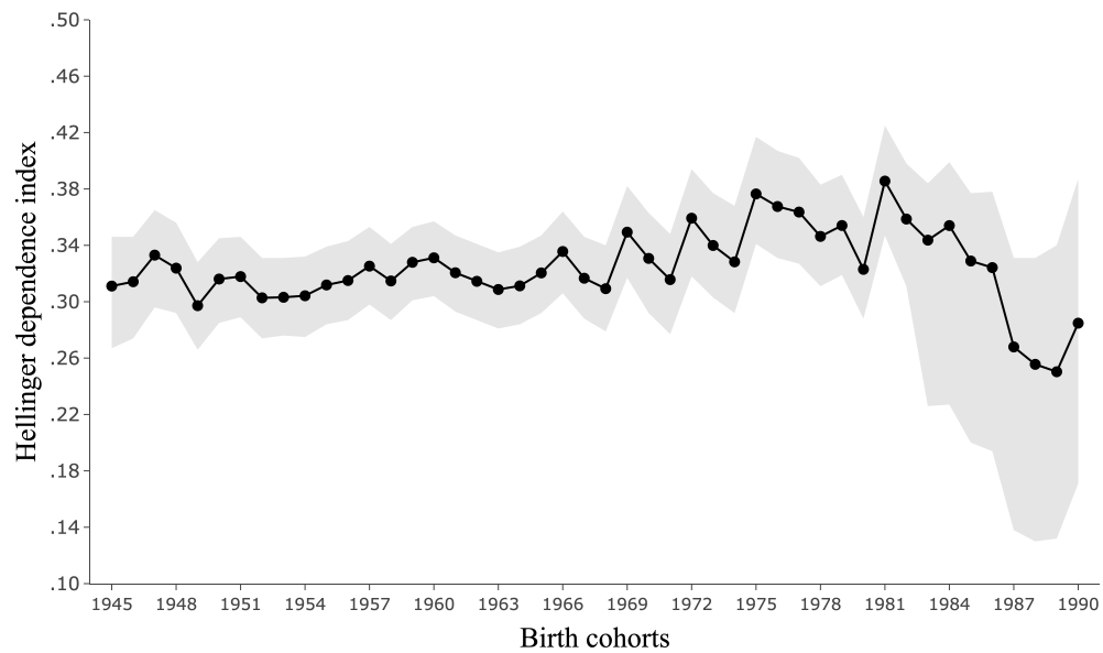
(B) Hellinger dependence index
