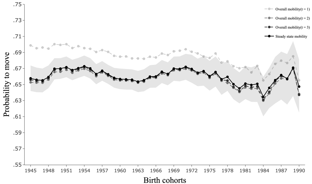
Figure A.6: Overall mobility ( OM_t ) across synthetic generations computed from samples of respondents age 30-64
