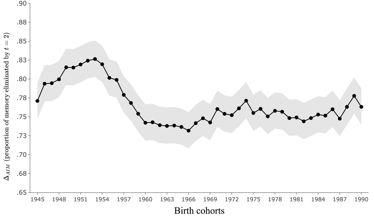
Figure 6: Rate of decay in aggregate intergenerational memory between generation t = 1 and t = 2
