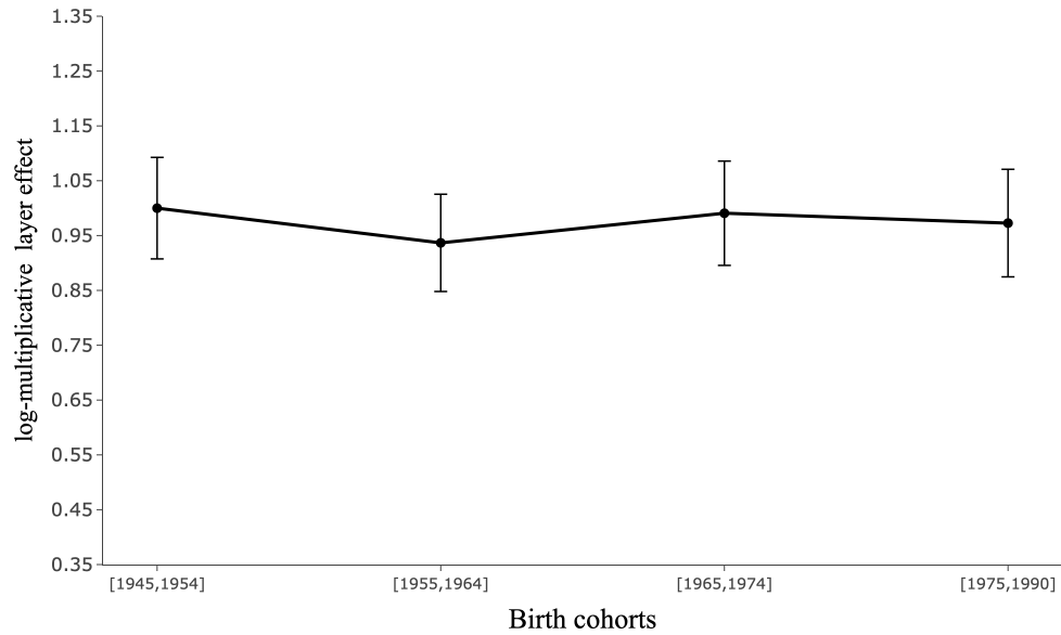
(B) Cohorts in ~10-year bins
