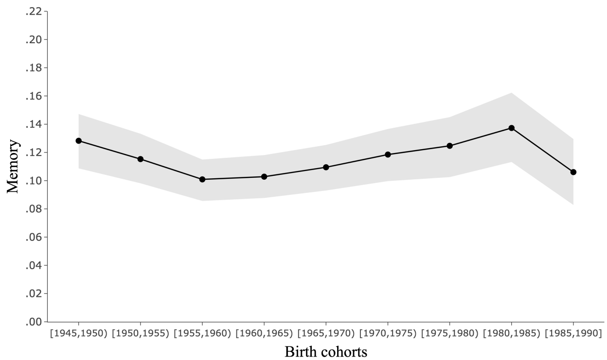
Figure G.6: Aggregate intergenerational memory at generation t = 1 ( AIM_1 ) based on 5-year cohort bins
