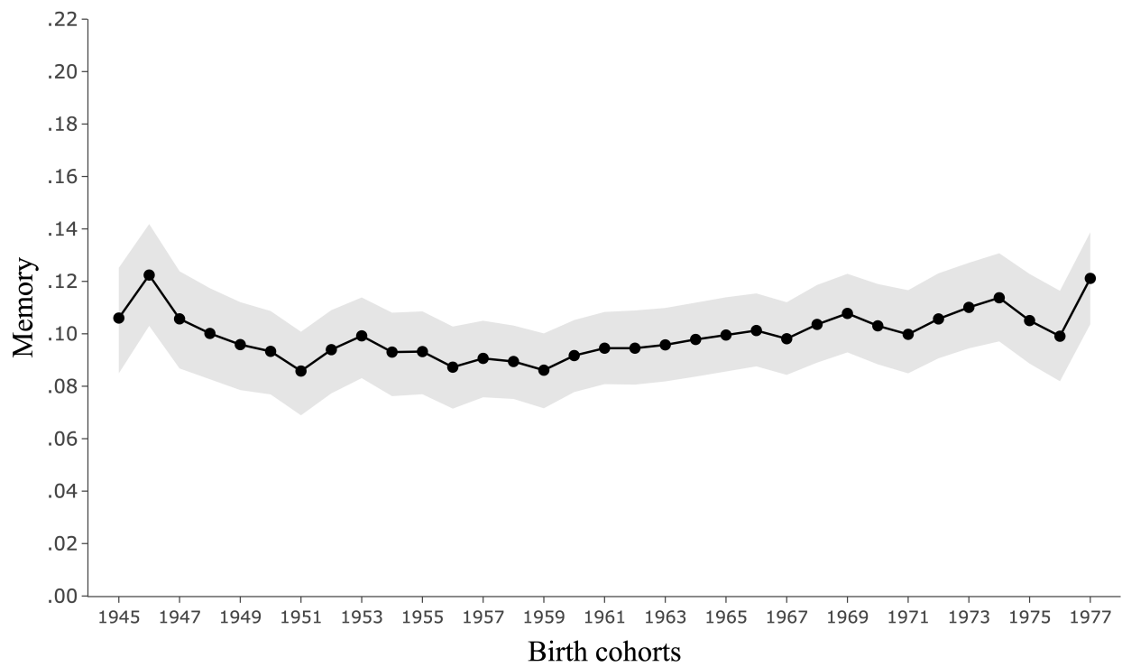
Figure E.3: Aggregate intergenerational memory at generation t = 1 ( AIM_1 ) based on father-daughter pairs
