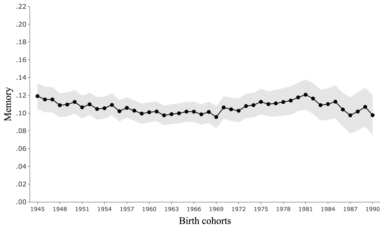
Figure F.3: Aggregate intergenerational memory at generation t = 1 ( AIM_1 ) based on White father-child pairs
