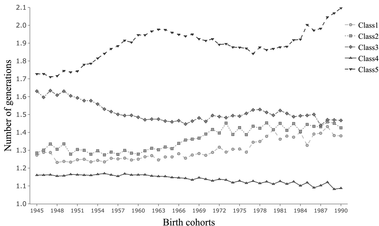
Figure C.3: Mean time to exit from each origin class ( MTE_i )
