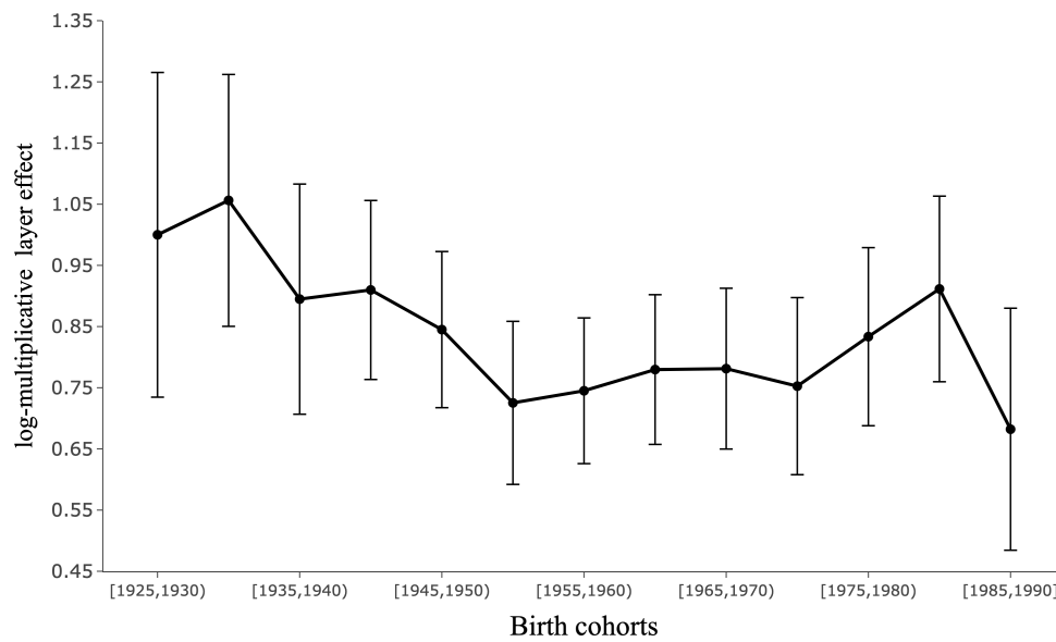
Figure H.4: Log-multiplicative layer effects based on cohorts born between 1925 and 1985
