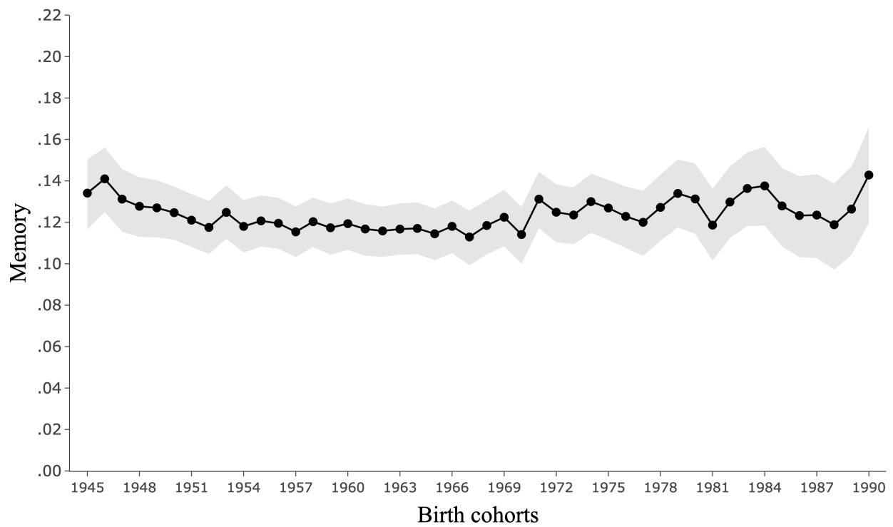
Figure B.15: Aggregate intergenerational memory at generation t = 1 ( AIM_1 ) based on Erikson and Goldthorpe (2010) typology
