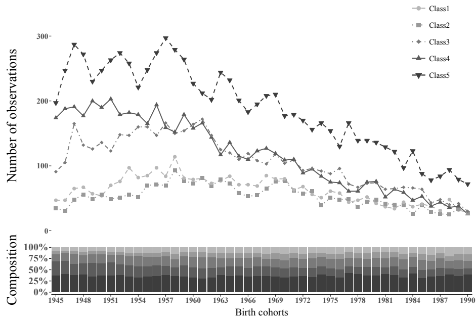
(B) Class origins of fathers
