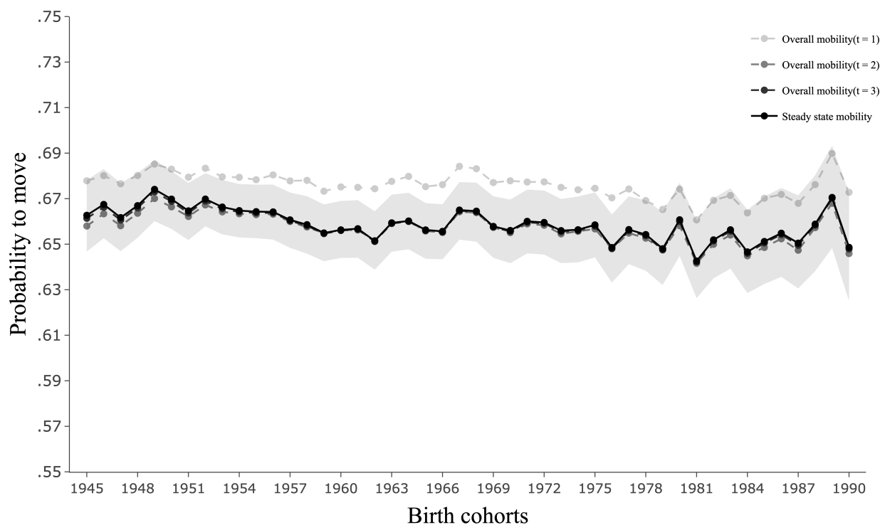
Figure B.10: Overall mobility ( OM_t ) across synthetic generations excluding farmers
