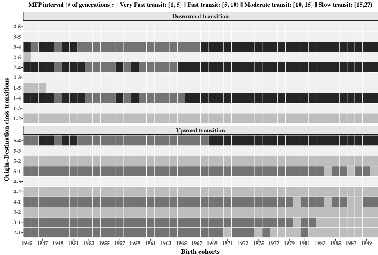
Figure D.2: Mean first passage time
