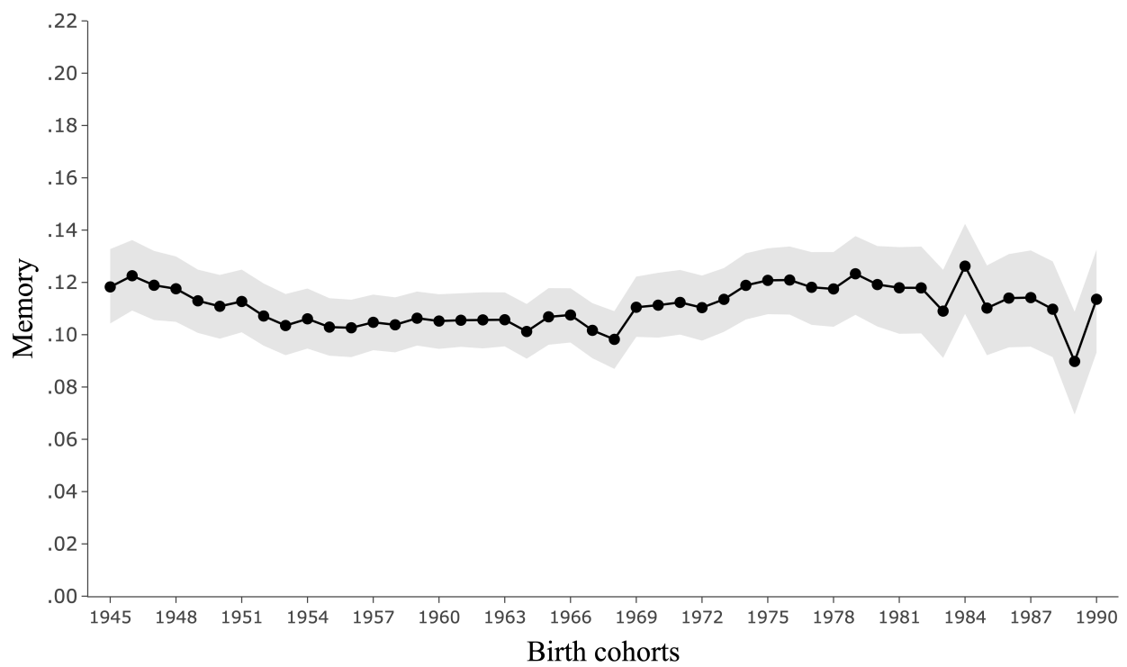
Figure B.11: Aggregate intergenerational memory at generation t = 1 ( AIM_1 ) excluding farmers
