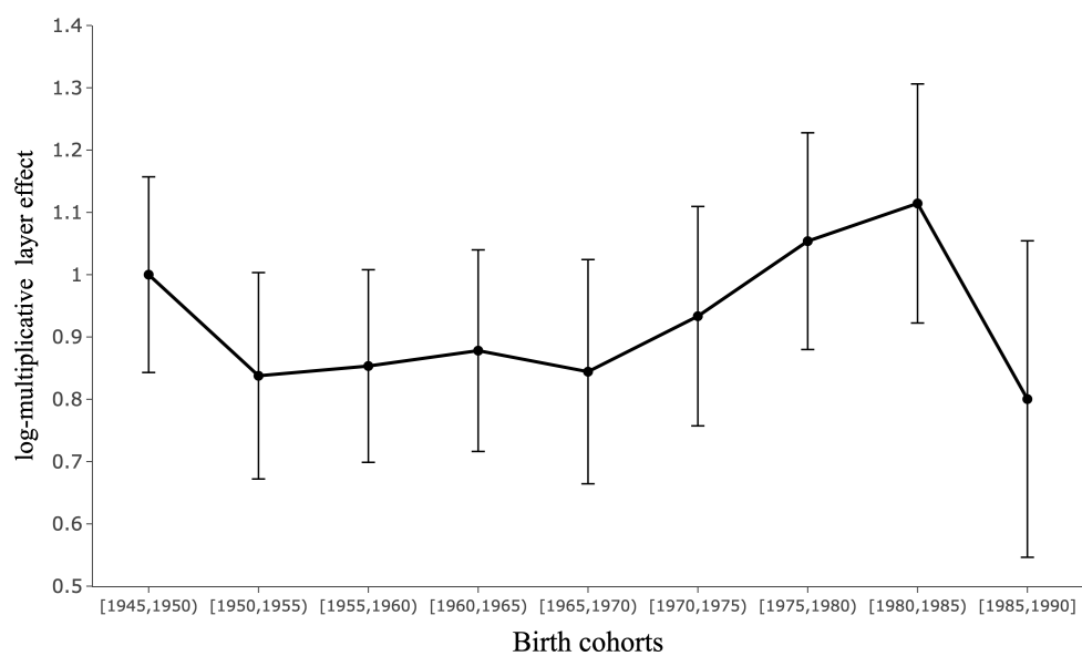
Figure E.8: Log-multiplicative layer effects based on father-son pairs
