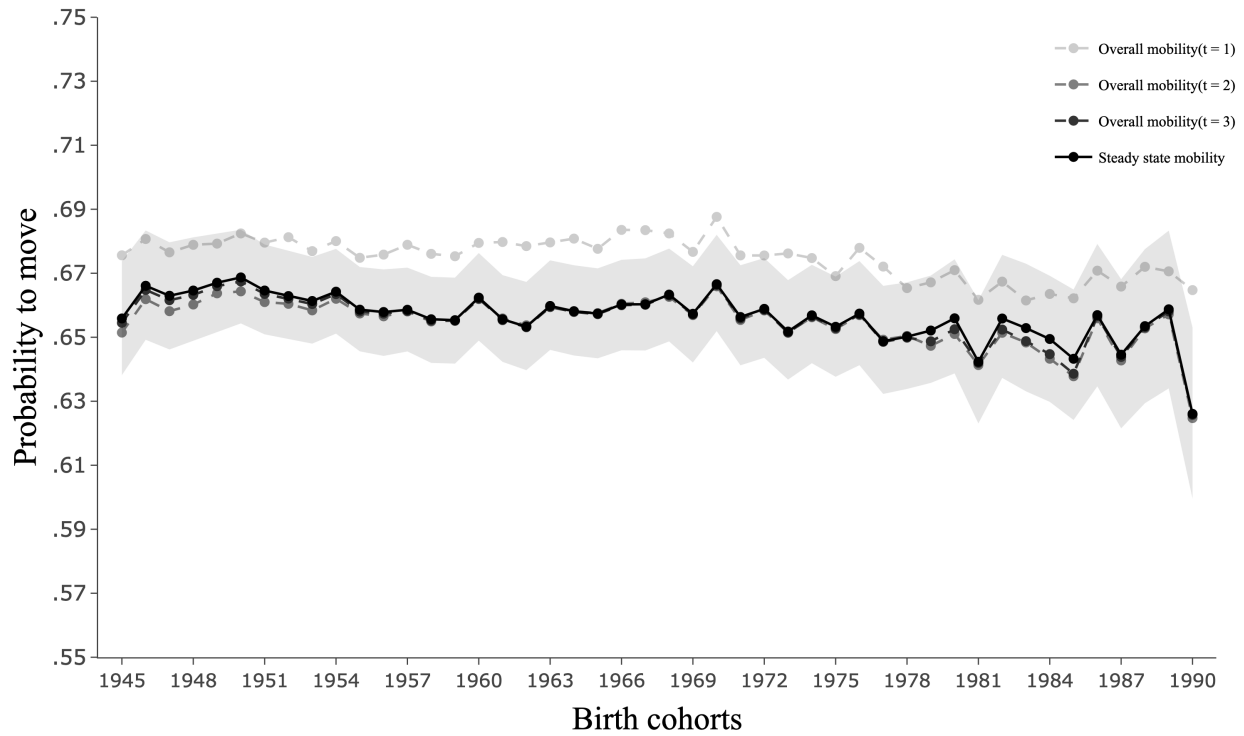
Figure B.14: Overall mobility ( OM_t ) across synthetic generations based on Erikson and Goldthorpe (2010) typology
