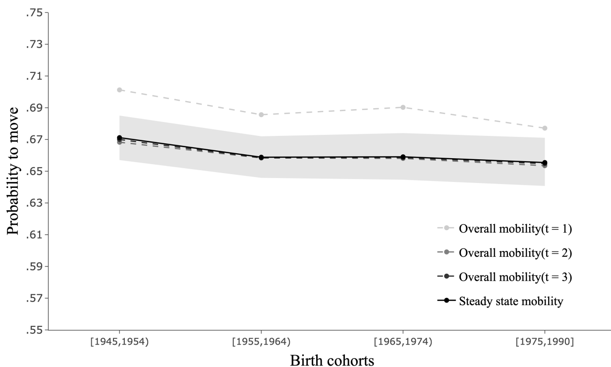
Figure G.2: Overall mobility ( OM_t ) across synthetic generations based on 10-year cohort bins
