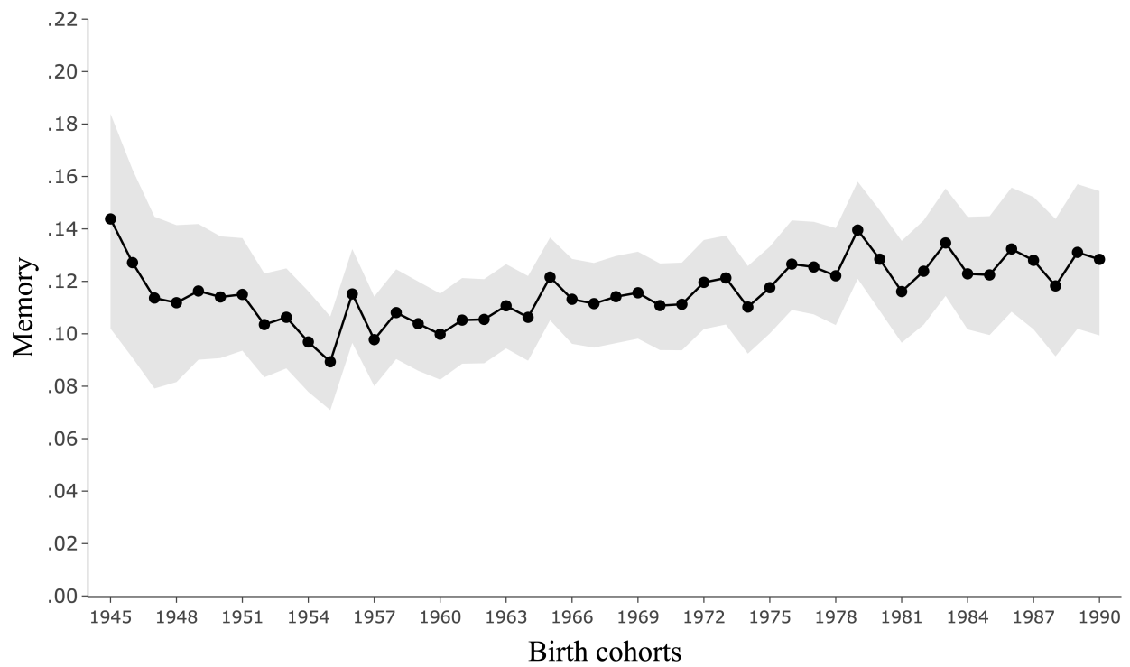
Figure E.15: Aggregate intergenerational memory at generation t = 1 ( AIM_1 ) based on parent with higher status-child pairs
