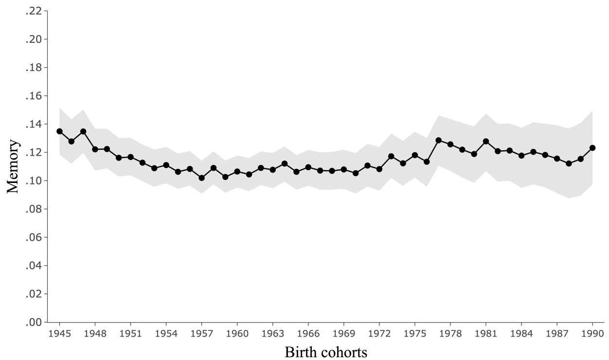
Figure C.4: Aggregate intergenerational memory at generation t = 1 ( AIM_1 )
