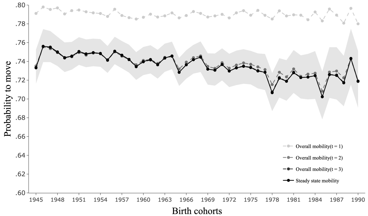
Figure B.6: Overall mobility ( OM_t ) across synthetic generations based on the Morgan (2017) typology
