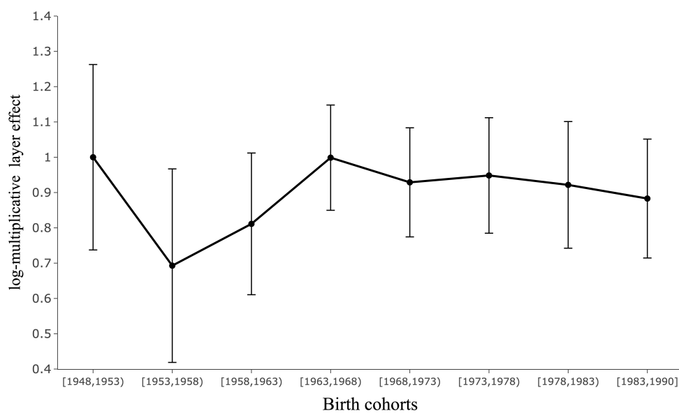
Figure E.12: Log-multiplicative layer effects based on mother-child pairs
