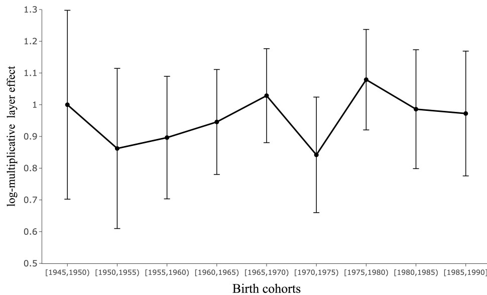
Figure E.16: Log-multiplicative layer effects based on parent with higher status-child pairs
