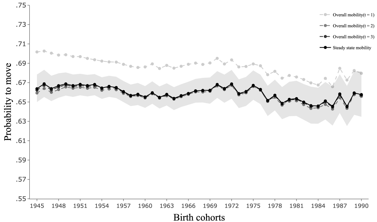
Figure A.2: Overall mobility ( OM_t ) across synthetic generations computed from samples of respondents age 25-64
