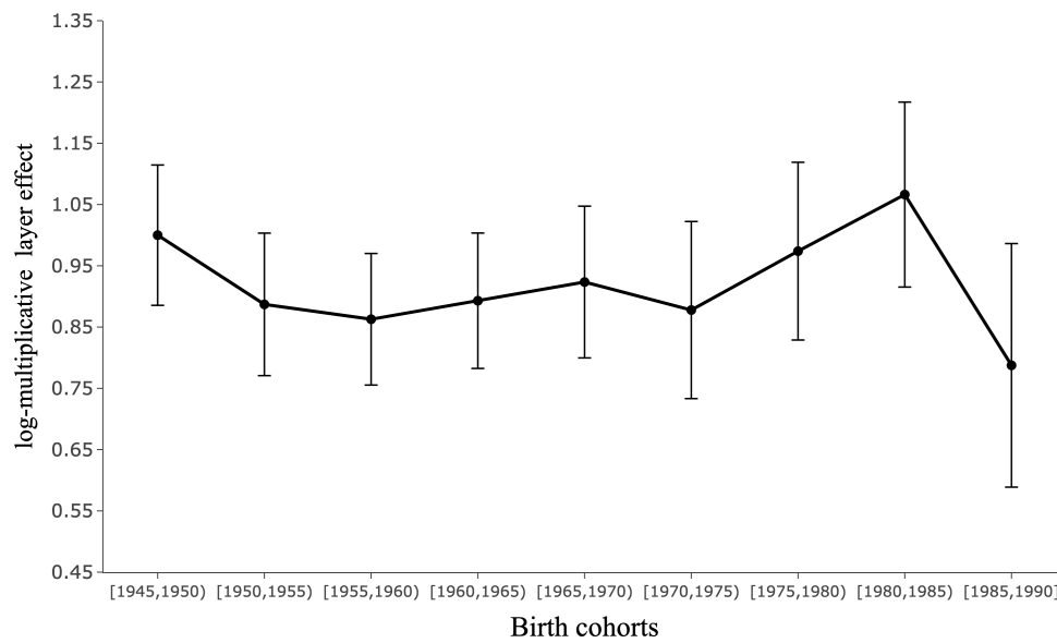
Figure A.4: Log-multiplicative layer effects computed from samples of respondents age 25-64
