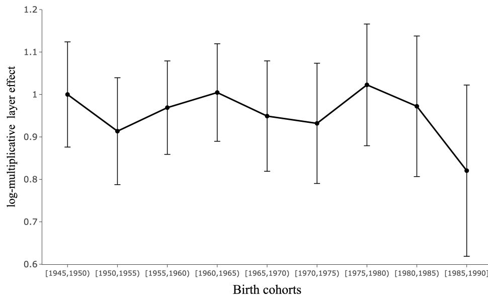
Figure B.4: Log-multiplicative layer effects based on the Pfeffer and Hertel (2015) typology
