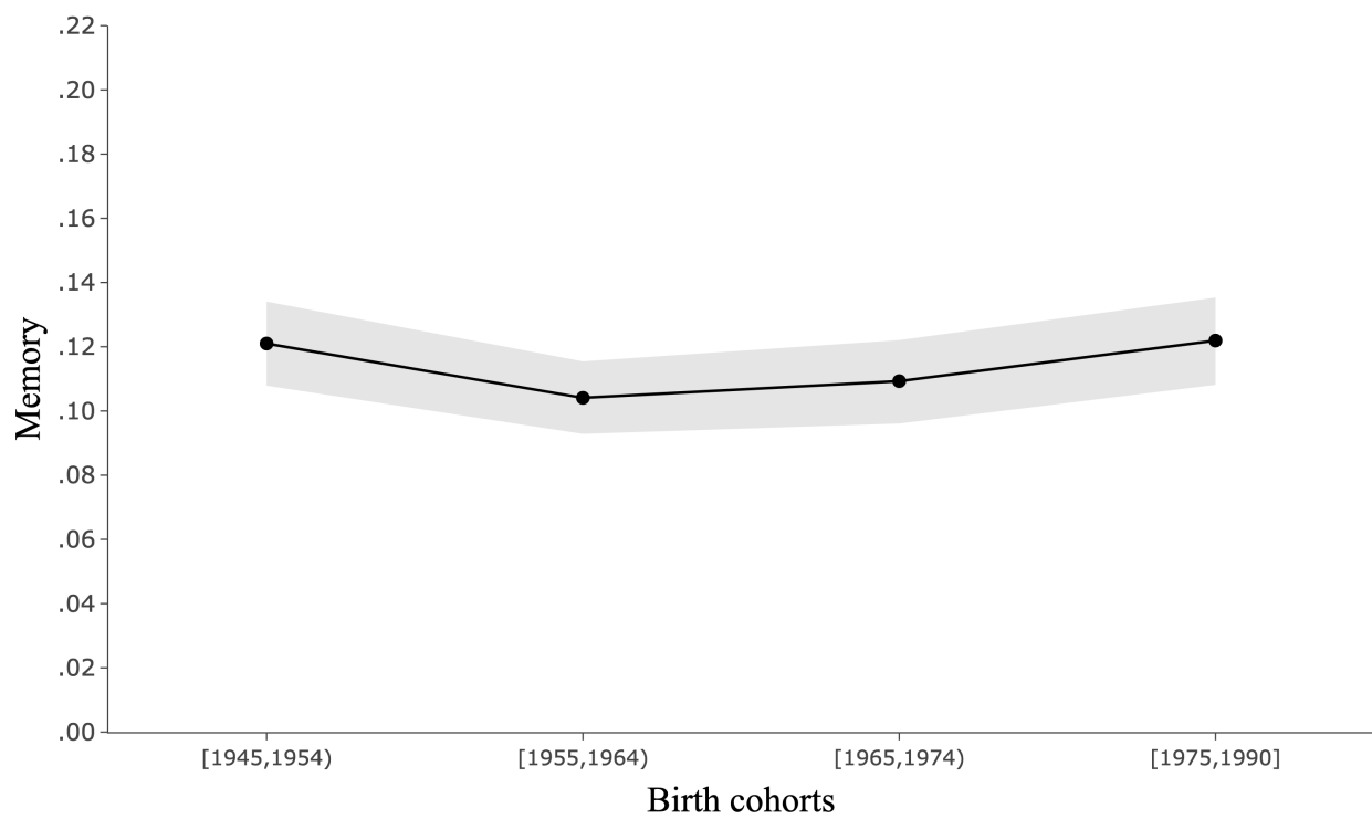
Figure G.3: Aggregate intergenerational memory at generation t = 1 ( AIM_1 ) based on 10-year cohort bins
