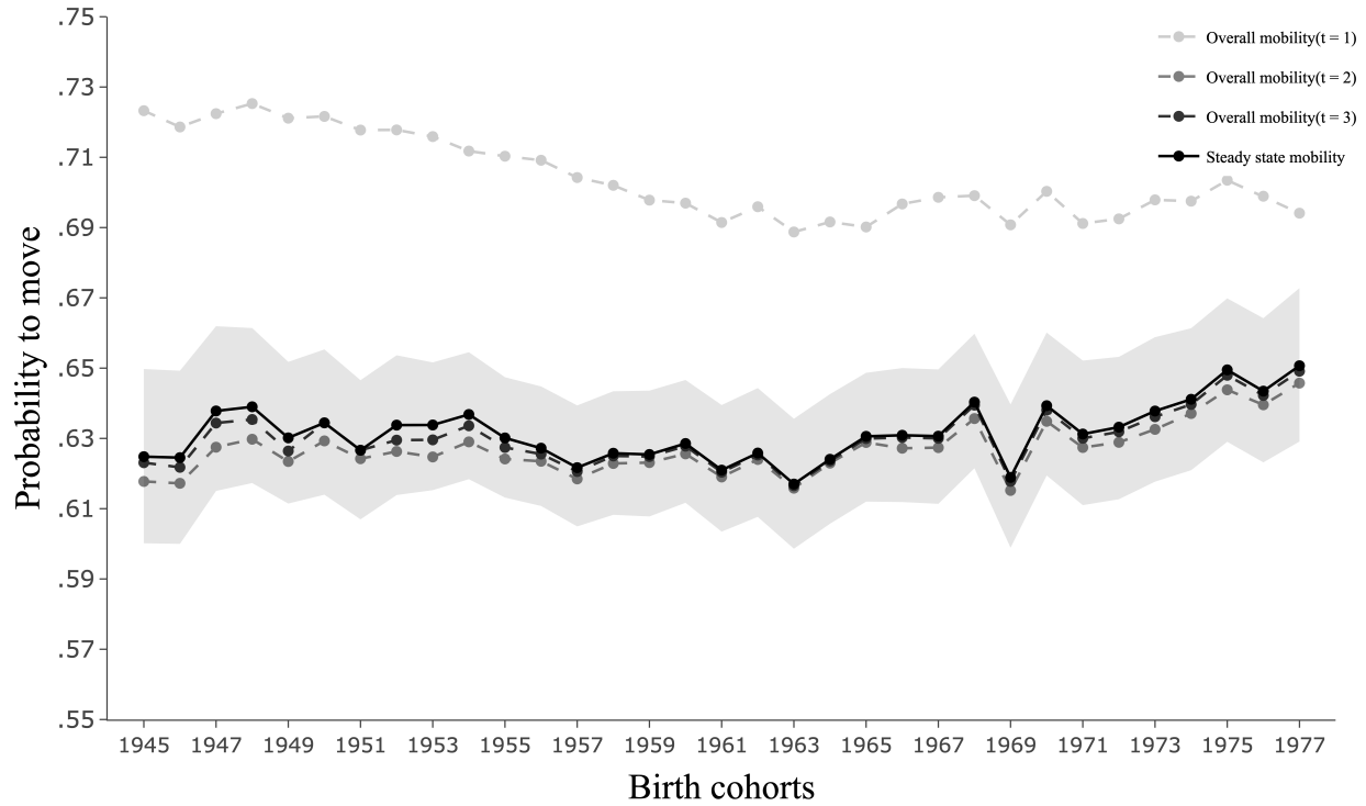
Figure E.2: Overall mobility ( OM_t ) across synthetic generations based on father-daughter pairs
