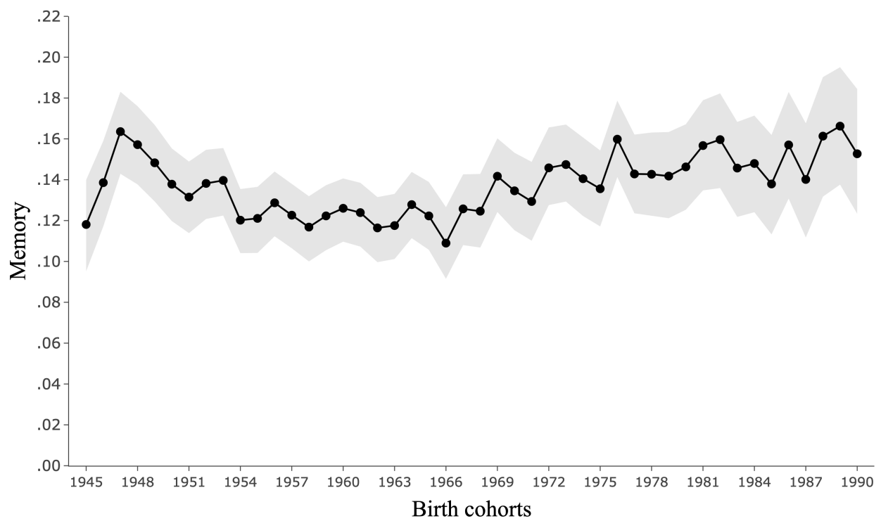
Figure E.7: Aggregate intergenerational memory at generation t = 1 ( AIM_1 ) based on father-son pairs
