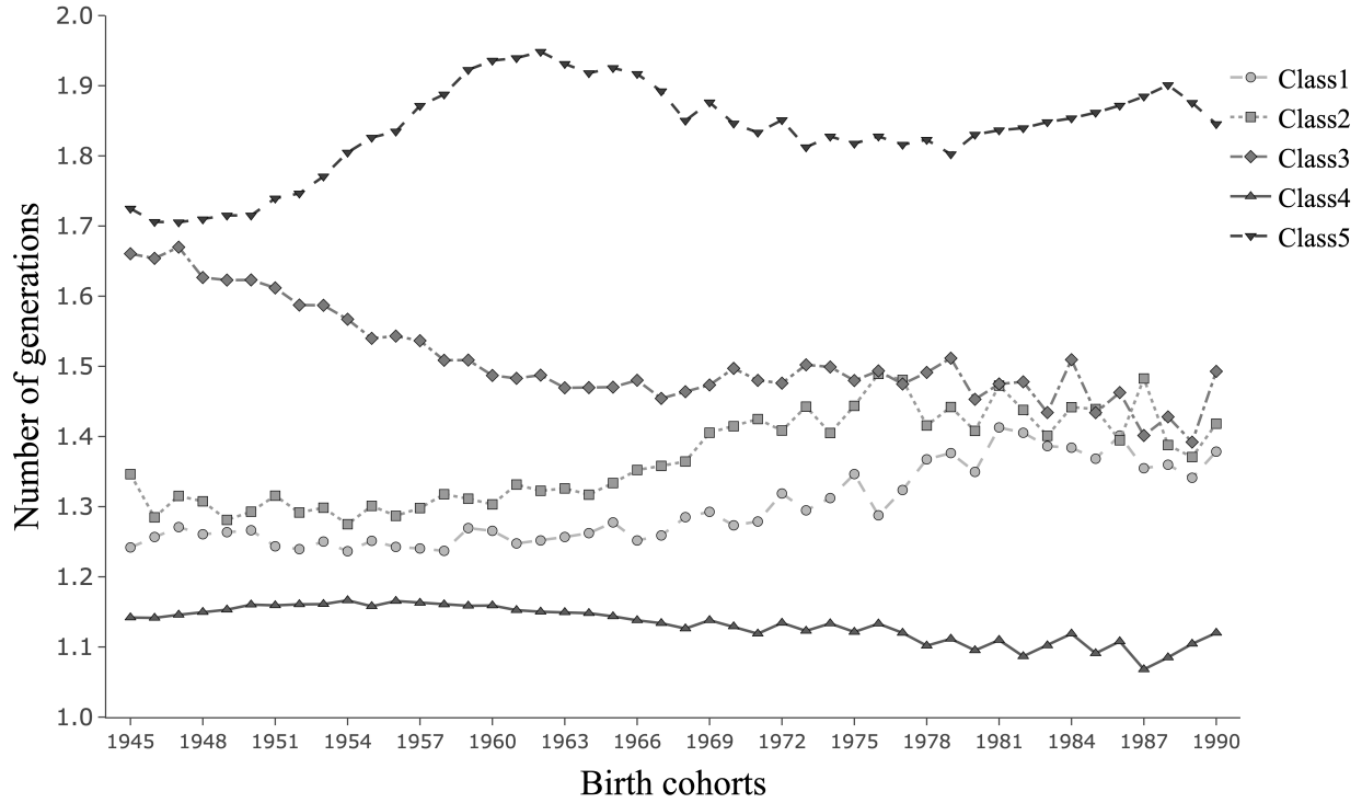
Figure 4: Mean time to exit from each origin class ( MTE_i )
