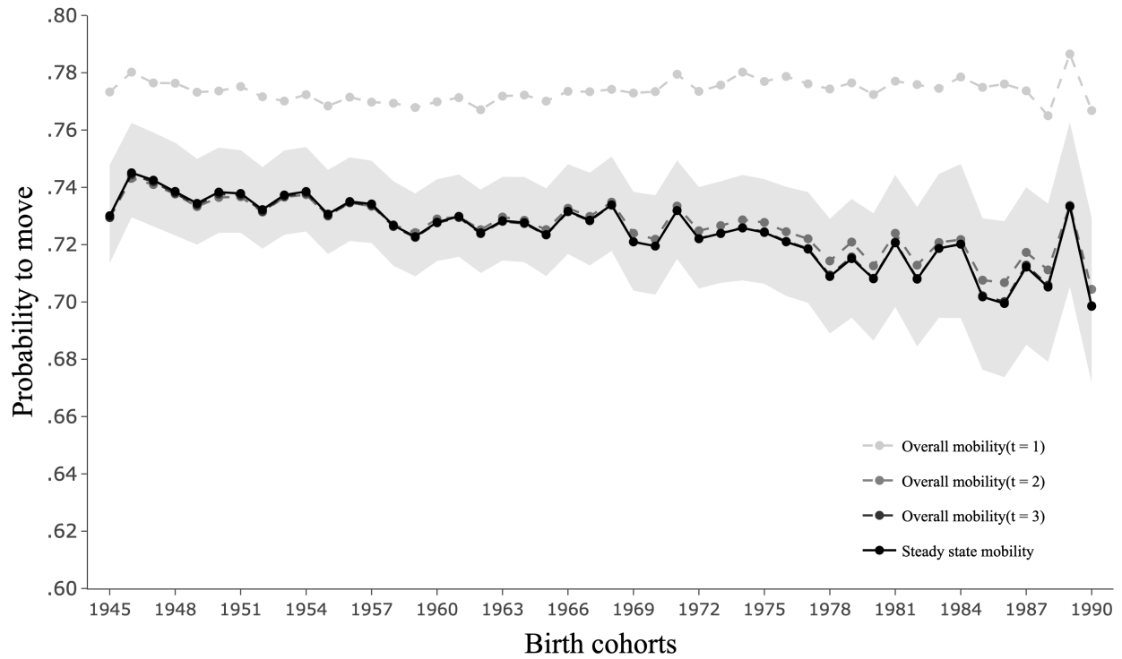
Figure B.2: Overall mobility ( OM_t ) across synthetic generations based on the Pfeffer and Hertel (2015) typology
