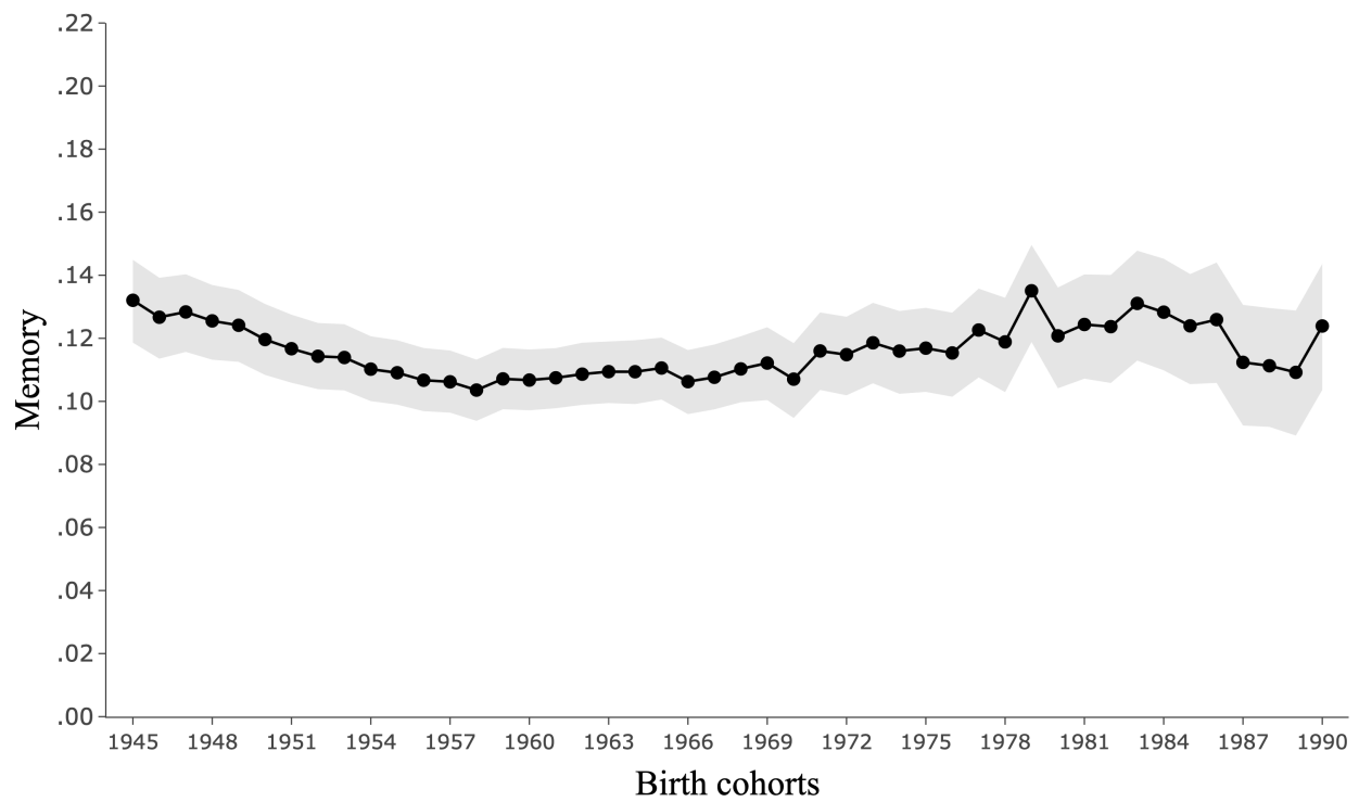
Figure A.3: Aggregate intergenerational memory at generation t = 1 ( AIM_1 ) computed from samples of respondents age 25-64
