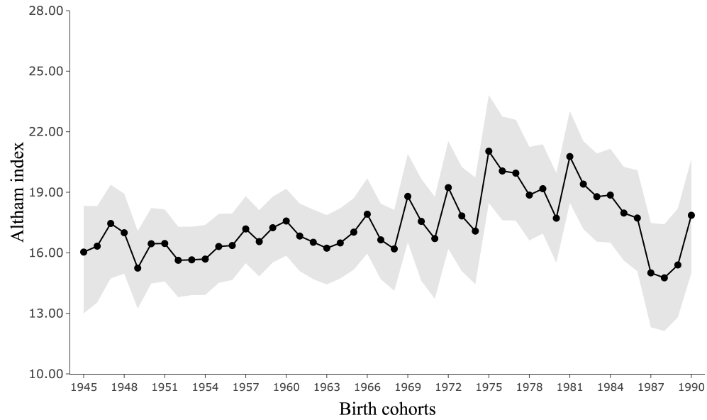
(A) Altham index
