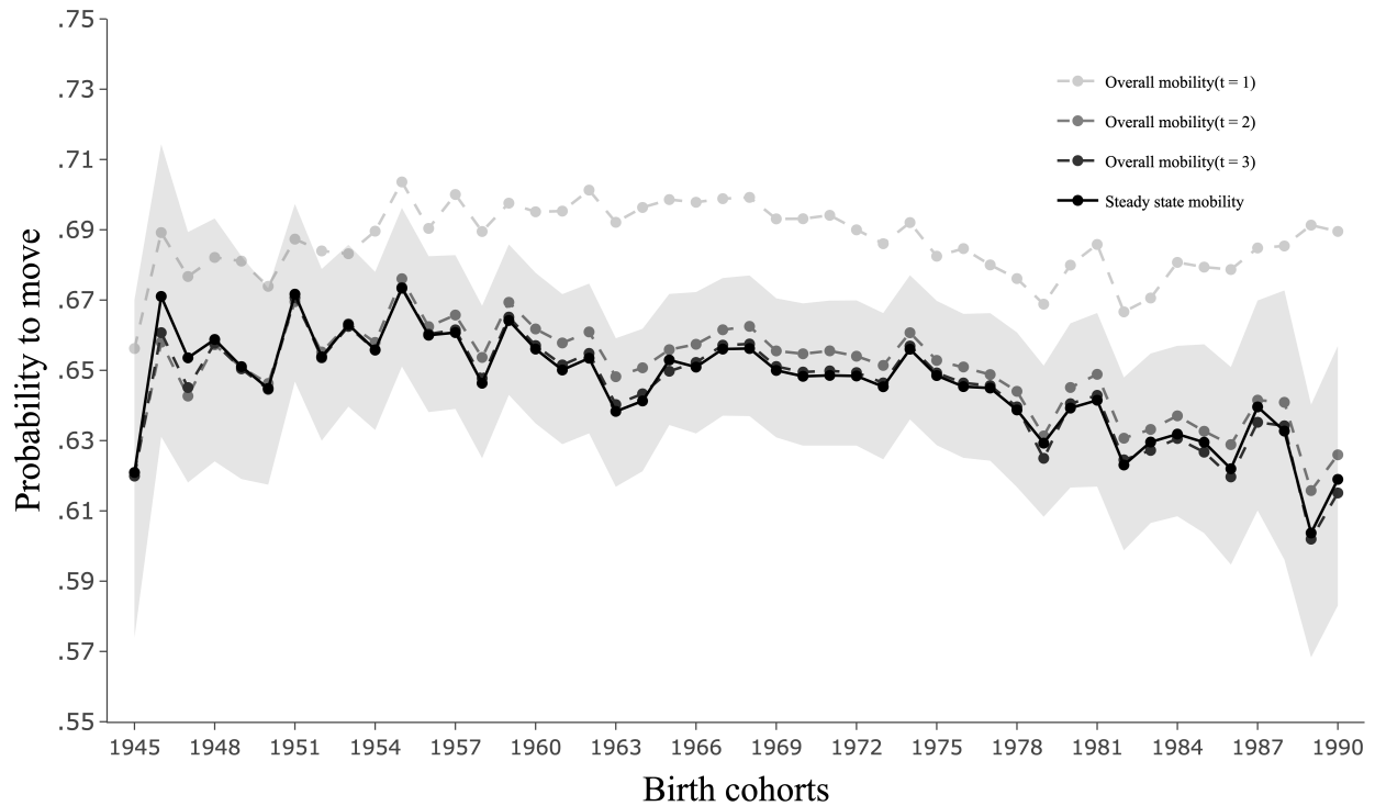
Figure E.14: Overall mobility ( OM_t ) across synthetic generations based on parent with higher status-child pairs
