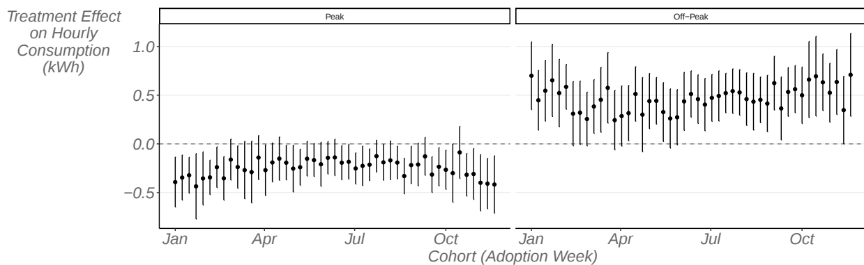
Figure A19: Cohort Specific Difference-in-Differences Estimate of IO Go
