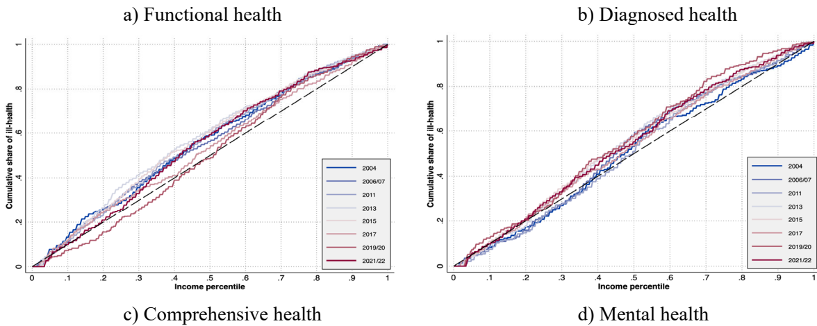
Figure 18. Concentration indices
