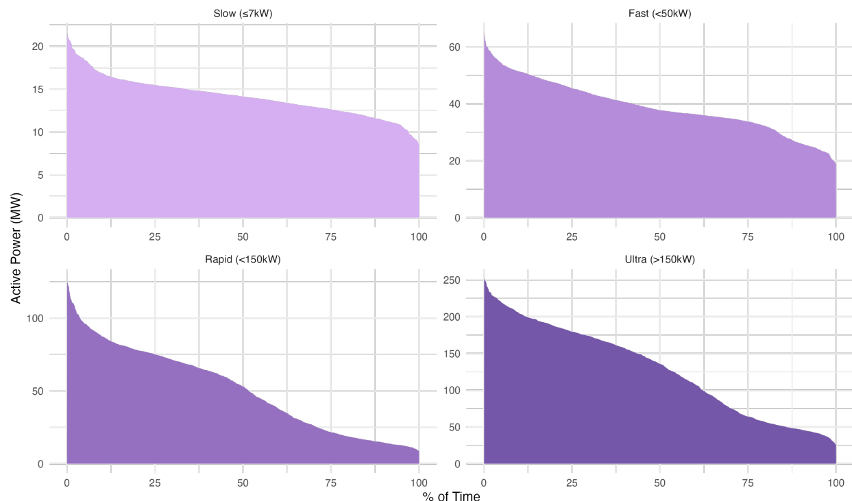
Figure A23: Load duration curve by charger speed
