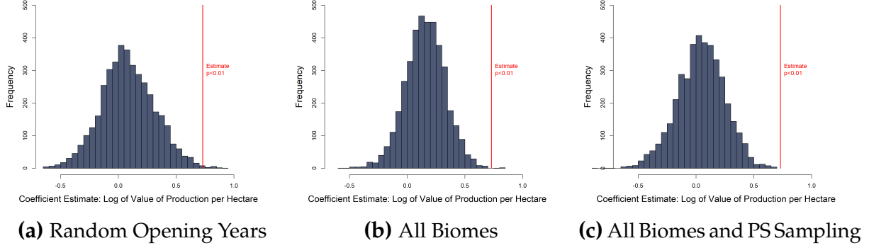
Figure 6: Falsification Tests
