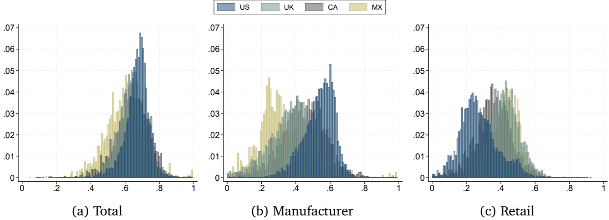
Figure 5: Markups Distributions
