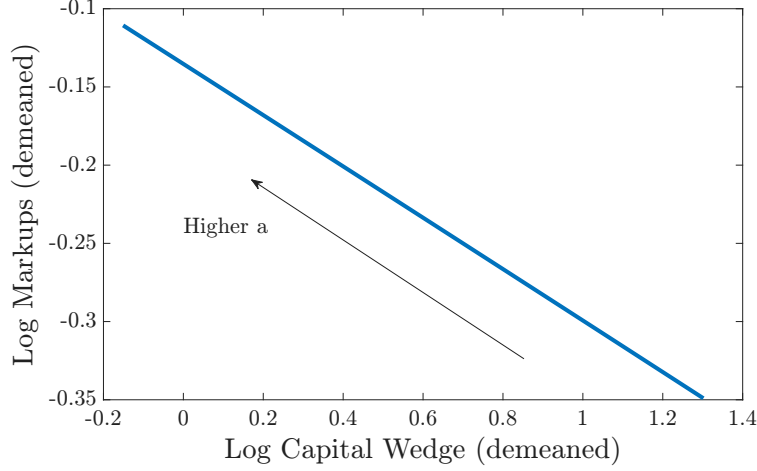
Figure 3: Markups and Constraint Tightness of Firms with Different Net Worth a but the Same Productivity z . This figure plots, for firms with the same productivity ( \log z at its mean) but different net worth a , their constraint tightness, measured as log capital wedges \log(1 + \tau_k) (demeaned, x-axis), and their log markup \log \mu (demeaned, y-axis). The model parameters are from the baseline calibration explained below.
