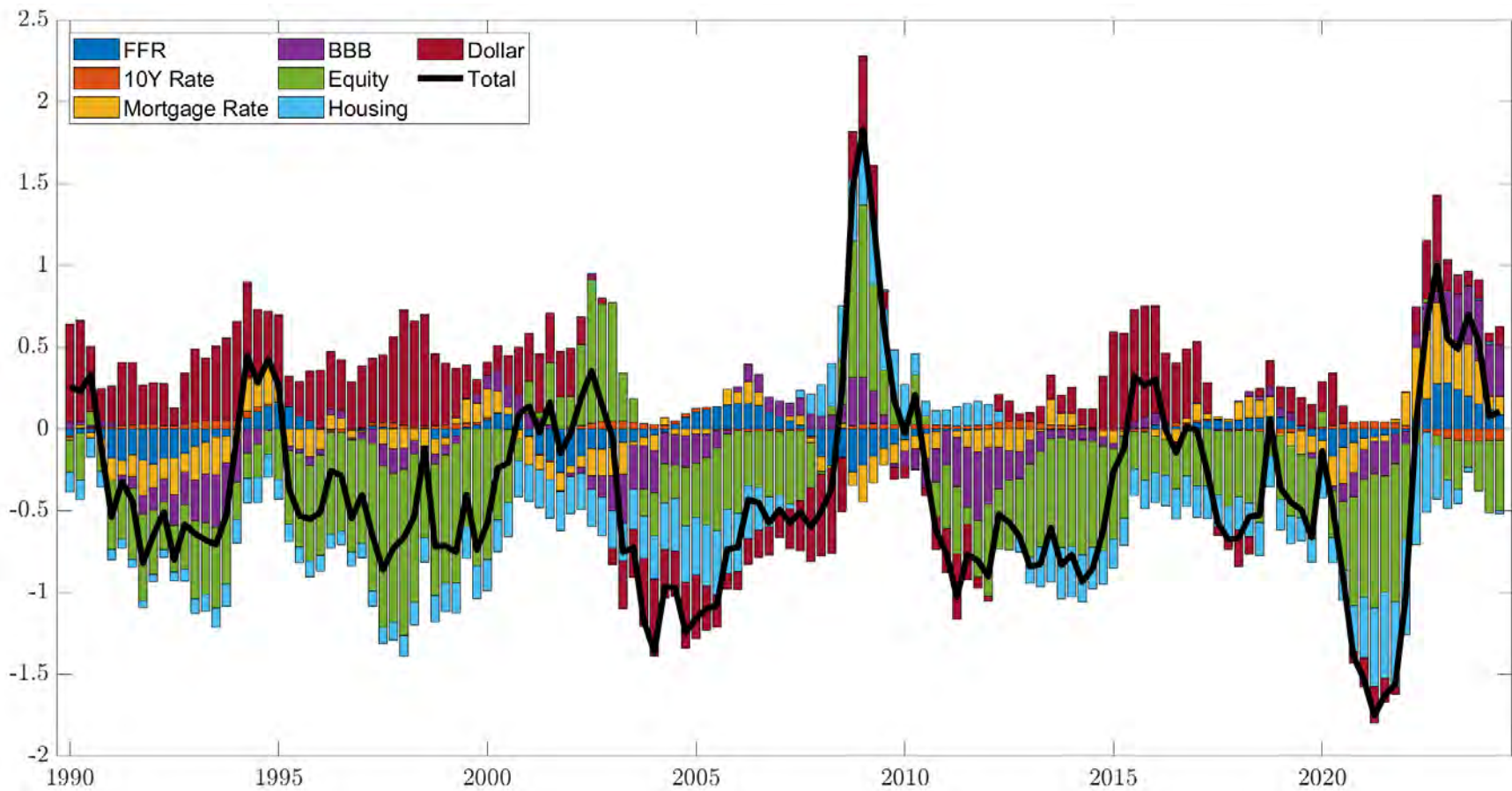
Figure 2: The FCI-G index (baseline measure with a three-year lookback) and its drivers over 1990Q1-2024Q2. Positive values imply a decrease in GDP growth in the next year. Source: Ajello et al. (2023)
