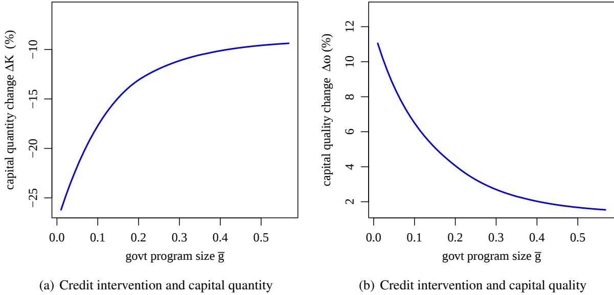
Figure A7: Credit intervention impact: Capital quantity vs. quality (under a larger \eta ). This figure illustrates how \bar{g} affects \Delta K_t and \Delta \omega_t in a crisis, under larger \eta . The calculation requires the pre-crisis \omega_{t-} which we set to the average value \bar{\omega} . This figure contrasts with Figure 2 in the main text.
