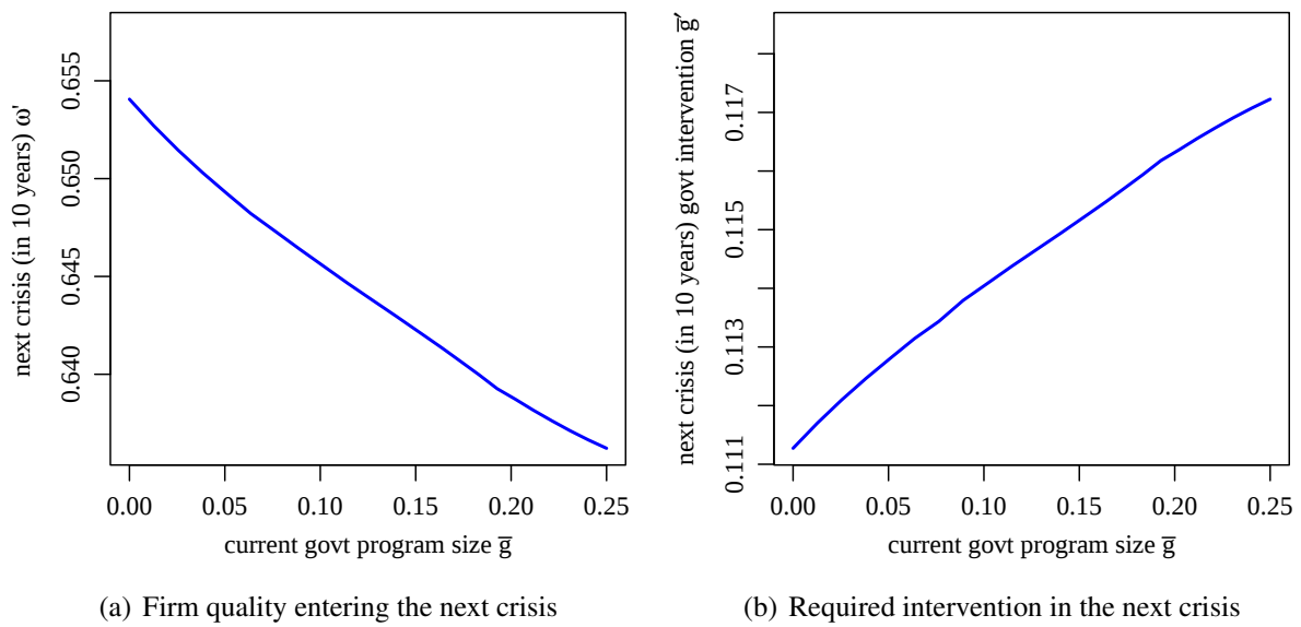
Figure A12: Intervention pass-through across crises (with type transition). We show how \bar{g} in the current crisis affects capital quality entering the next crisis, \omega' , and intervention needed, \bar{g}' , in the next crisis to contain output drop to be y . This limit y is set so that the starting point of the curve in Panel B, denoted by \bar{g}'(\bar{g} = 0) , is the same as Figure 6 in the main text. The next crisis happens ten years after the current one. Agents expect no intervention (pass-through is only due to forward propagation). The current crisis happens at \omega equal to the average value of \omega_t in the laissez-faire economy.
