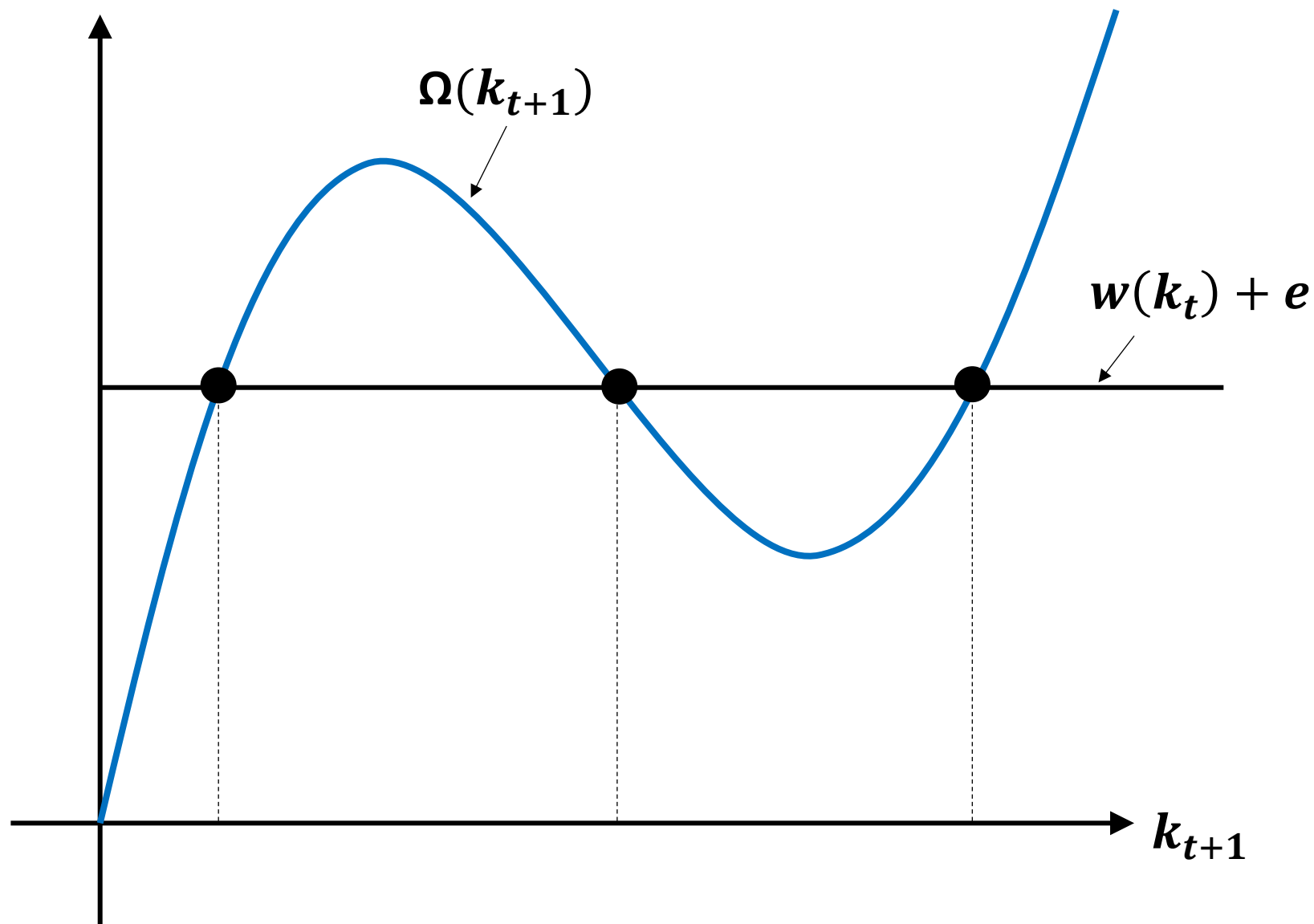
Figure 1: Existence of multiplicity of momentary equilibria
