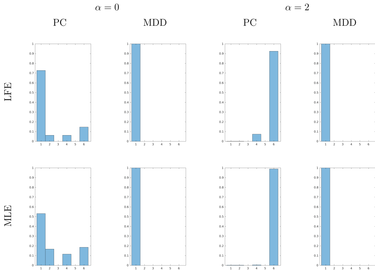
Figure A-1: DISTRIBUTION OF \hat{p} , HORIZON h = 4 , T = 500
