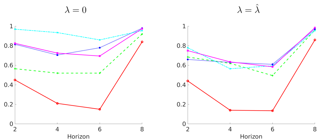
Figure A-4: Selection of LP versus VAR IRF Estimate
