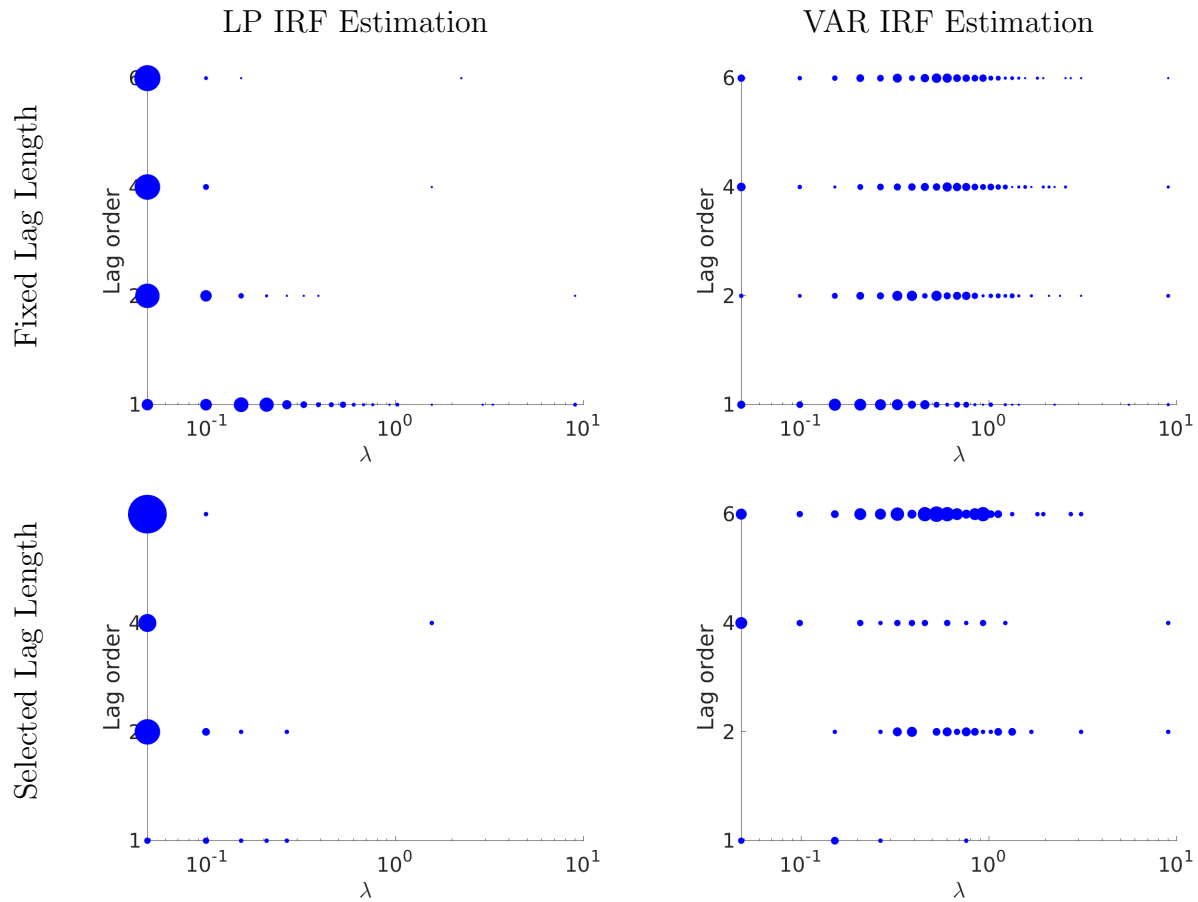
Figure A-3: Distribution of Selected Hyperparameter, h = 6 .
