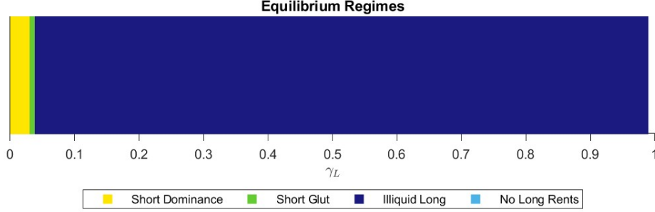
Figure 6: Equilibrium Cases as a function of \gamma_L under Limited Transactability
