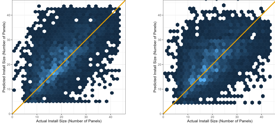
Figure C.1: Density plot of Google Sunroof-method predicted (y-axis) and actual (x-axis) installed system capacity sized using (left) actual consumption and (right) using assigned closest consumption bin, both inclusive of rebound. The diagonal represents correct predictions of the optimal installation size.
