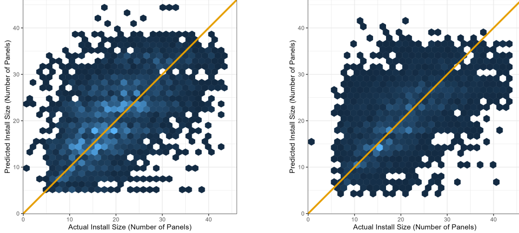
Figure B.2: Sizing model accuracy. Density plot of Google Sunroof-method predicted (y-axis) and actual (x-axis) installed system capacity for (left) purchased systems and (right) leased systems. The diagonal represents correct predictions of the optimal installation size.
