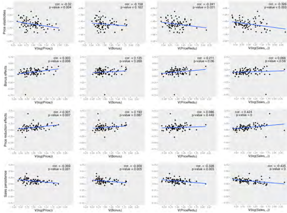
Figure 2: Scatter plots of 2sCOPE-MG store-specific estimates on within-store regressor variations
