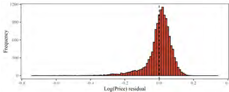
Figure 1: Histogram of the distribution of log price residuals
