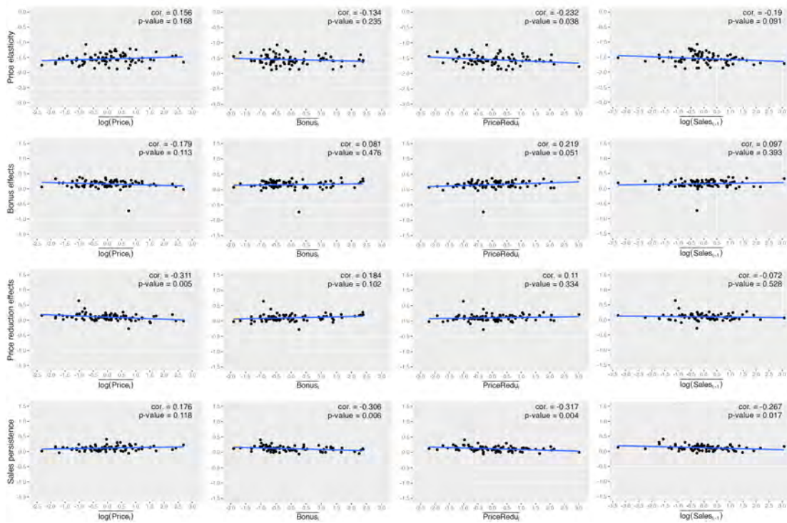
Figure W.1: Scatter plots of 2sCOPE-MG store-specific estimates on store-specific mean of regressors in a dynamic panel data model with lagged sales as regressors
