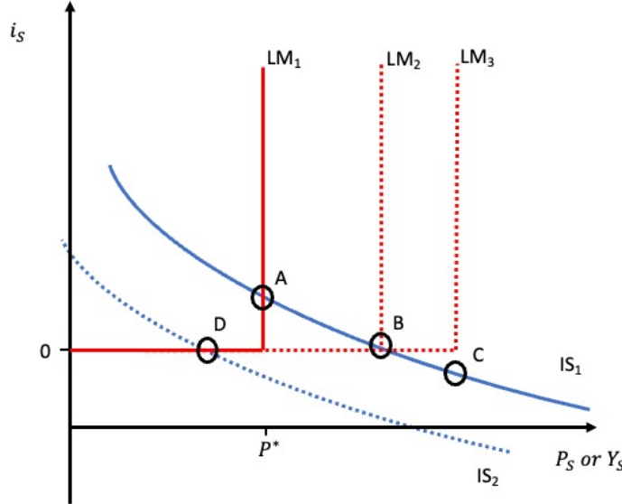
Figure 6: Liquidity Trap
