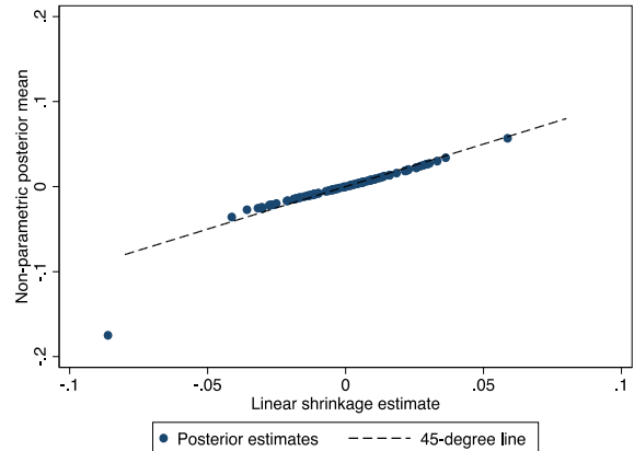
(ii). Linear shrinkage accounting for precision-dependence
