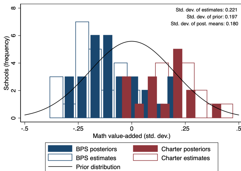
Figure 1: Empirical Bayes estimates of school value-added in Boston
