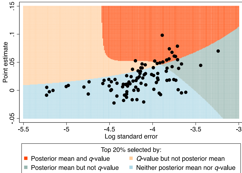
Figure 6. Selection frontiers for empirical Bayes decision rules
