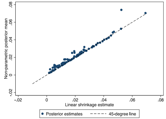
(ii). Linear shrinkage accounting for precision-dependence
