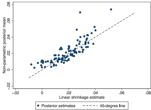
(i). Linear shrinkage ignoring precision-dependence
