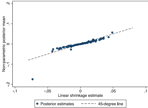
(i). Linear shrinkage ignoring precision-dependence
