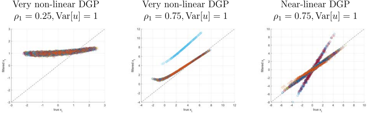
Figure 5: Partial filter with a quadratic observation equation and misspecification: Filtered state \hat{x}_t vs. true x_t for 100 different samples for varying degrees of persistence \rho_1 .
