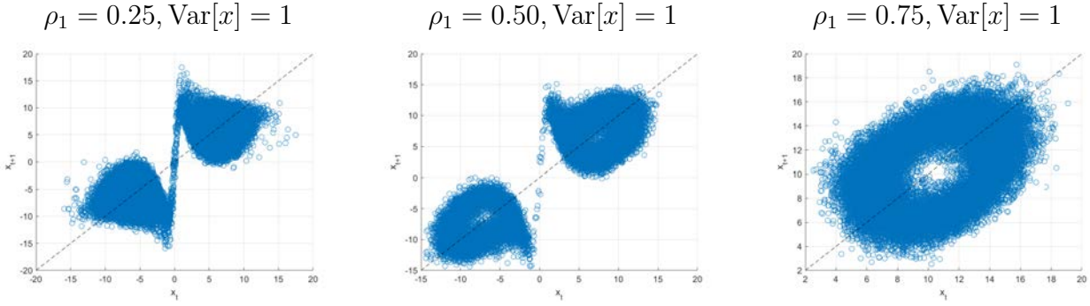
Figure A.6: Linear observation equation, non-linear state equation with cosine forcing term for varying degrees of persistence \rho_1 . True state vs. observation with T=25,000 observations.
