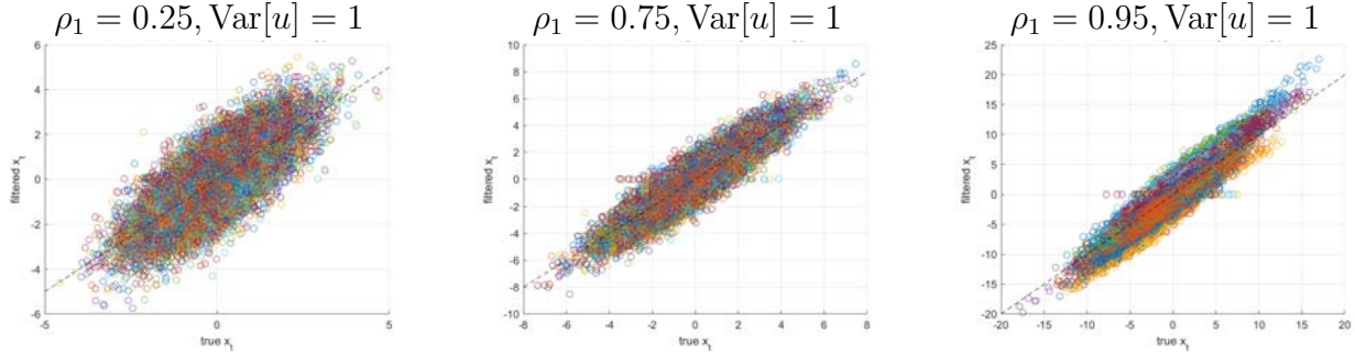
Figure 2: Partial filter in the fully linear case with misspecification: Filtered state \hat{x}_t vs. true x_t for 100 different samples for varying degrees of persistence \rho_1 .
