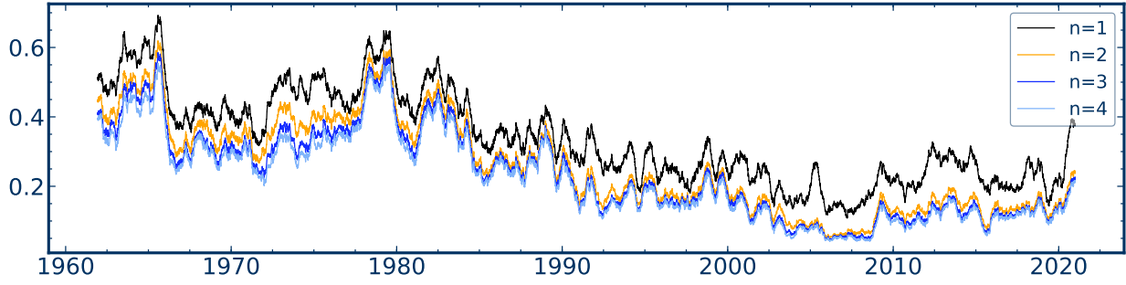
Figure 15: Unexplained variation by the first 4 KR factors
