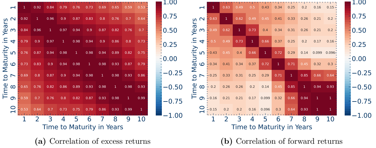
Figure 9: Correlation matrices of discount bond excess returns and forward returns
