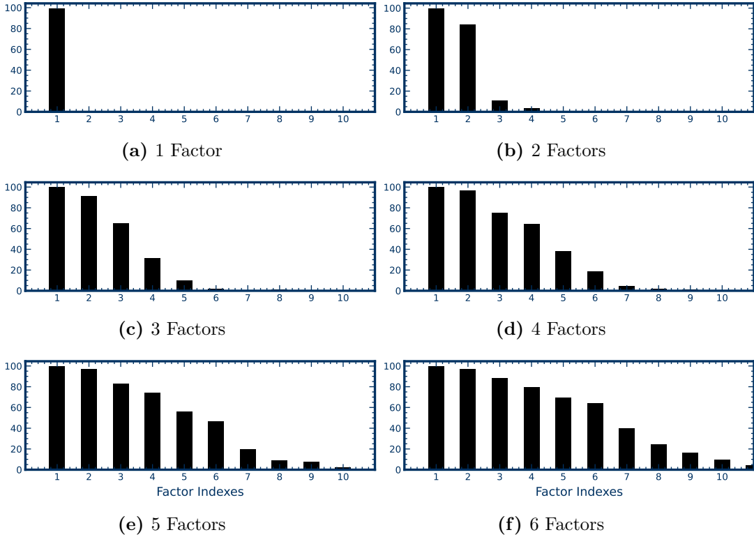
Figure 3: Frequency (%) of factors selected by LASSO
