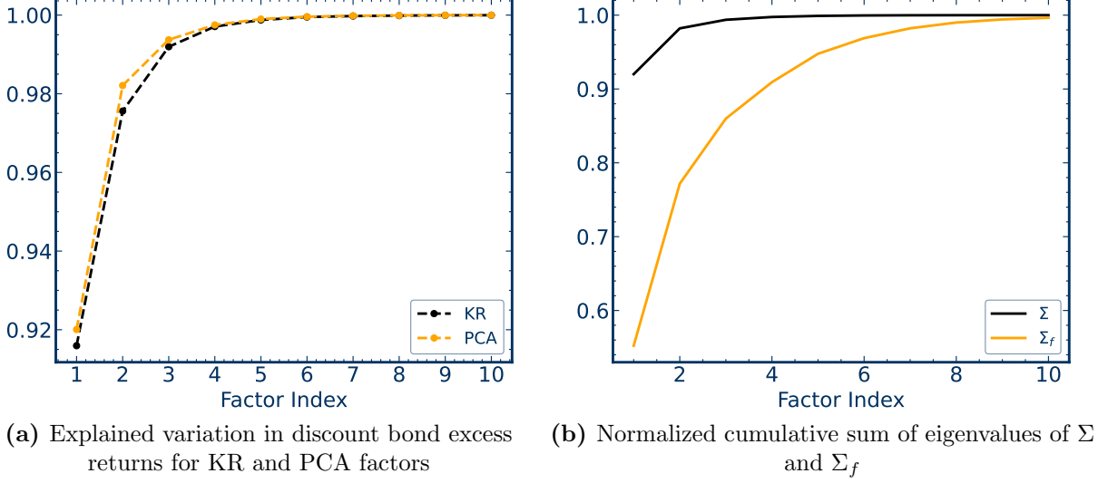
Figure 8: Explained variation and eigenvalue structure for different number of factors
