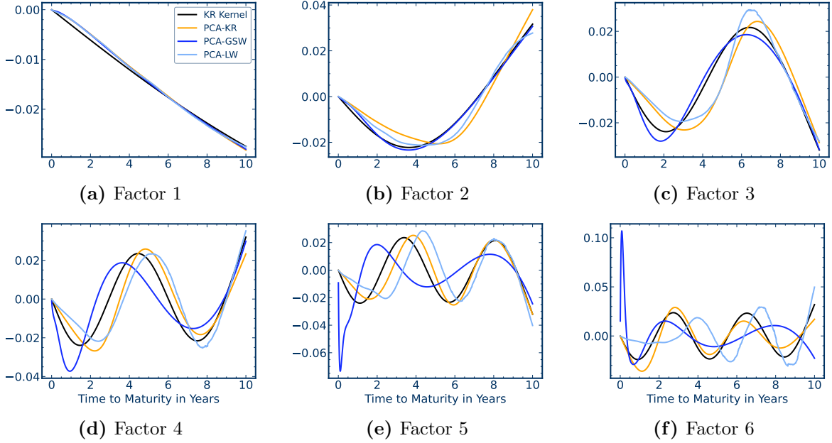
Figure 5: PCA factor loadings of KR, GSW and LW discount bond excess returns
