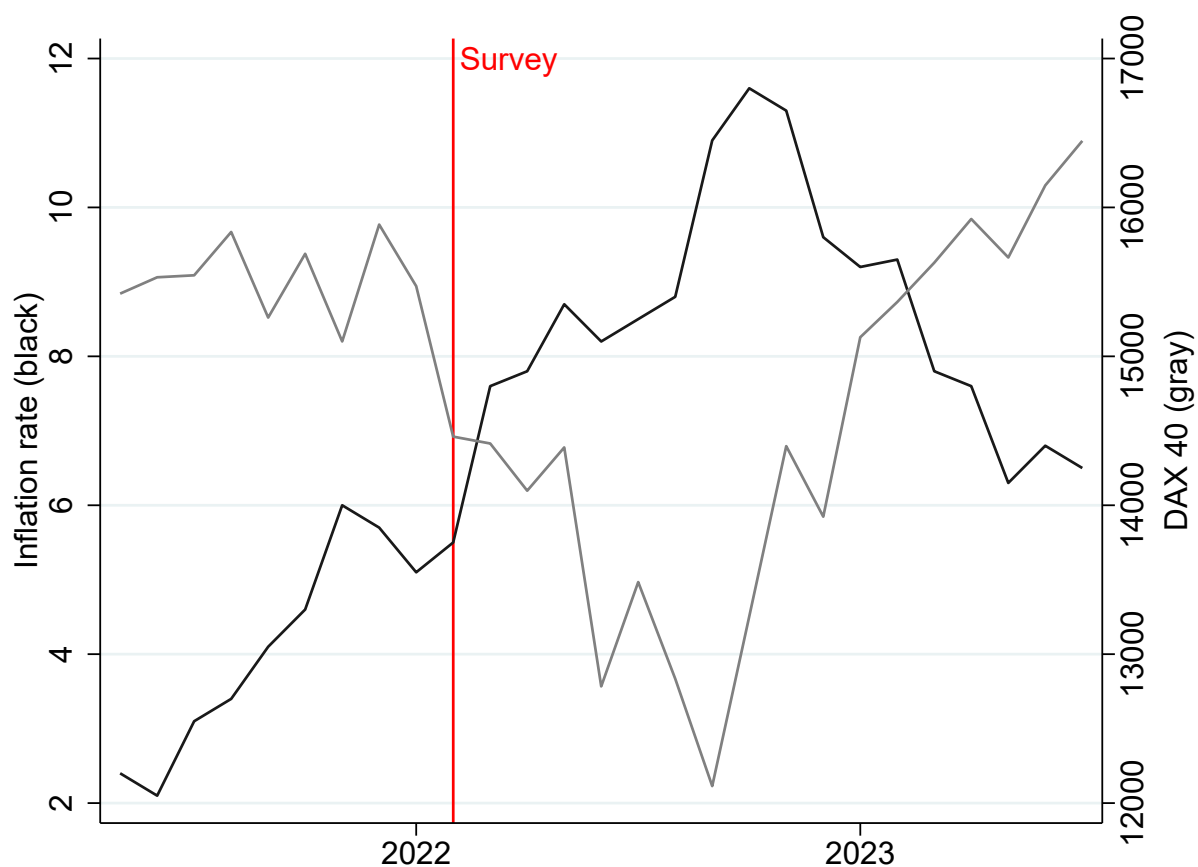
Figure A2: Inflation and stock returns around survey participation
