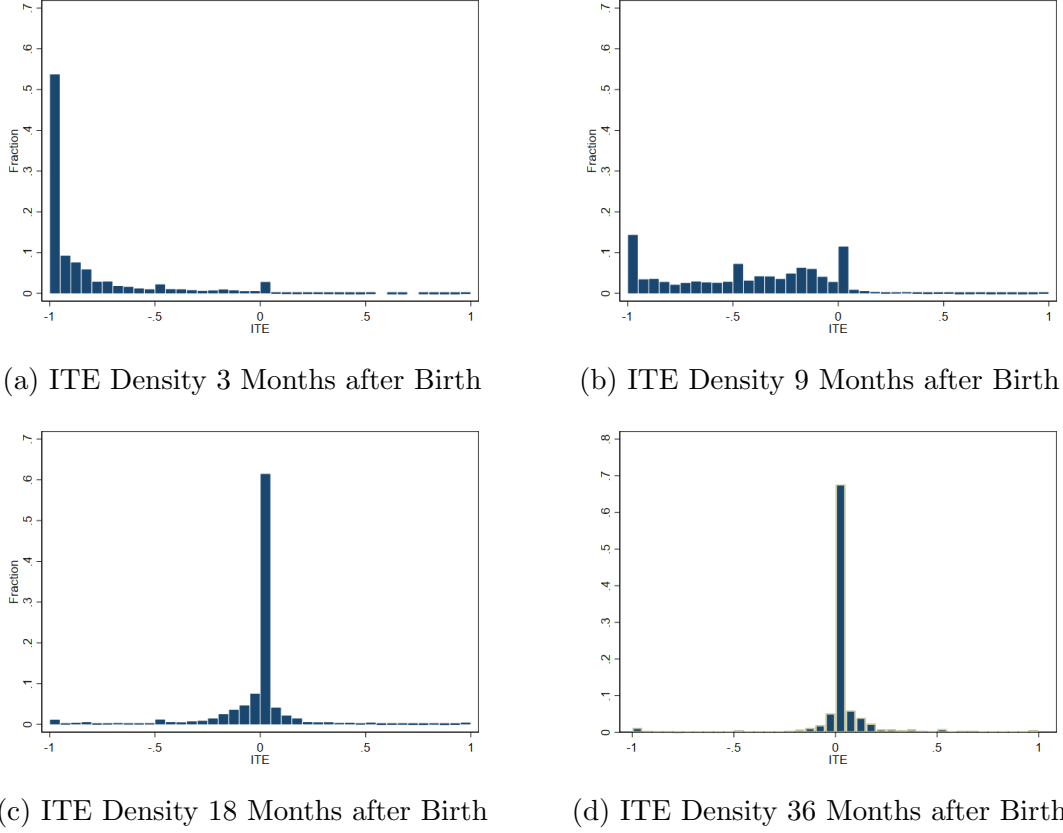
Figure 3: \widehat{seaITE} Density
