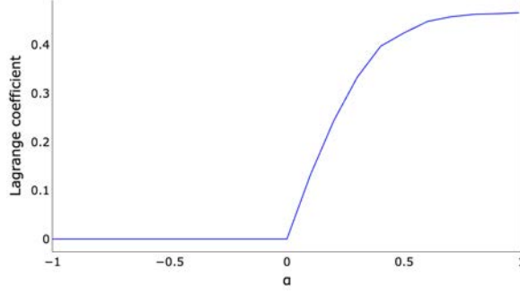
Figure 6. \nu as a function of \alpha in the example with uniformly distributed likelihood ratio and \theta = \frac{1}{2} .
