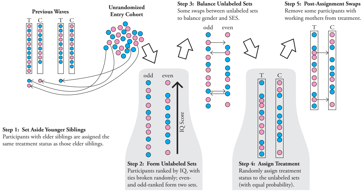
Figure 1: Graphical Description of the Randomization Procedure
