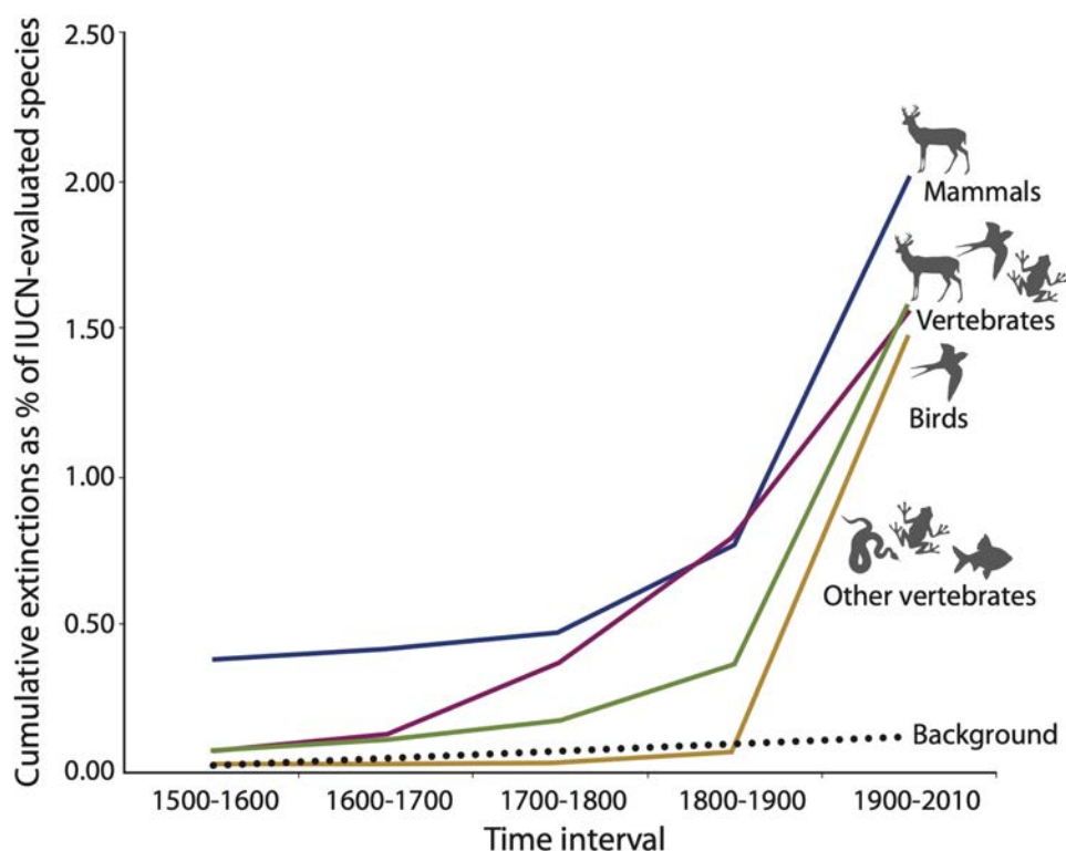
Figure 2: Conservative Count of Vertebrate Species Listed as Extinct, Extinct in the Wild and Possibly Extinct by IUCN (2012). Source: Ceballos et al. (2015).
