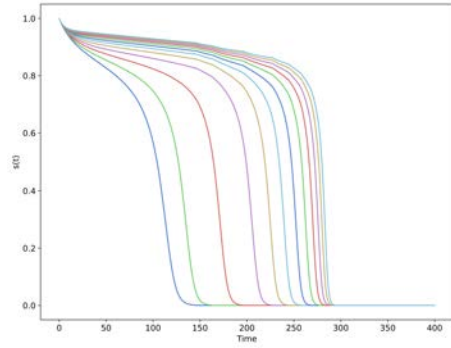
(a) Solution of the differential equation for different r values
