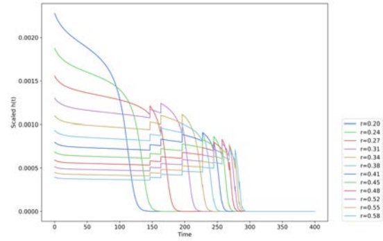
(b) h(t) for different r values
