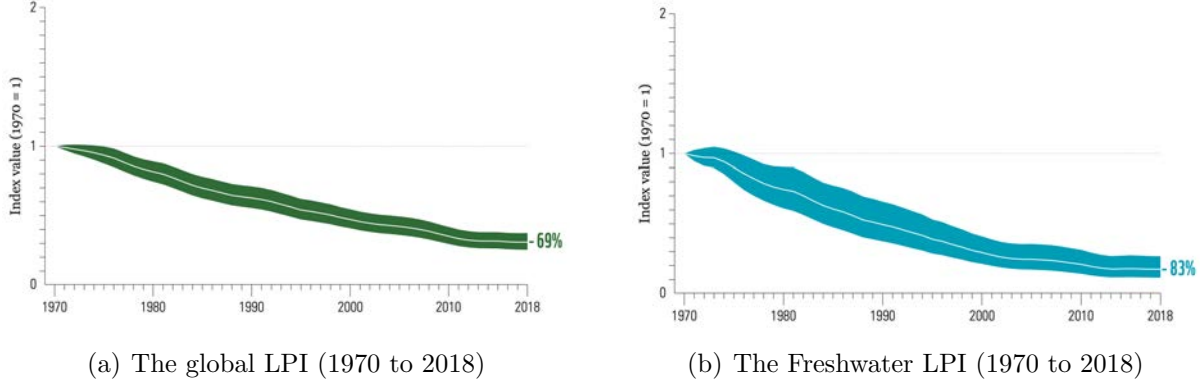
Figure 3: Living Planet Index Source: Almond et al. (2022).
