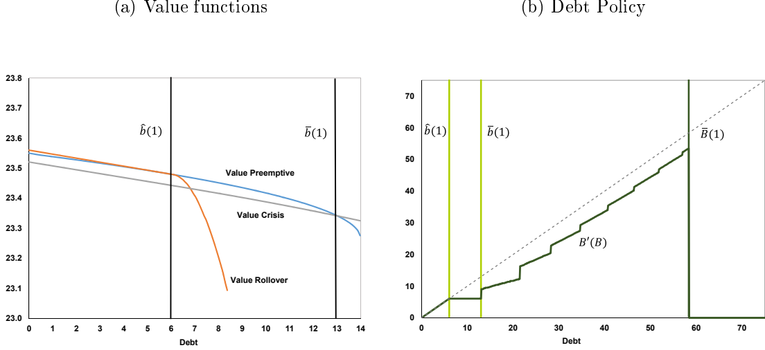
Figure 1: Value functions and optimal debt policy
