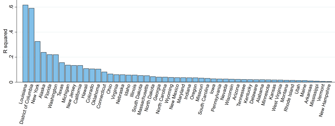
Figure C.2: R^2 of regression for each region r of \partial(\omega_r - \bar{\omega})/\partial m_{ih} on \{\partial(\omega_s - \bar{\omega})/\partial m_{ih}\}_{s \in \mathcal{S}}
