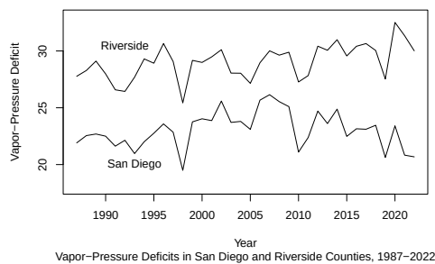
Figure 2(h): Vapor-Pressure Deficit: Riverside and San Diego Counties
