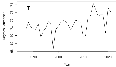
Figure 2(a): Maximum Temperature in California by Year
