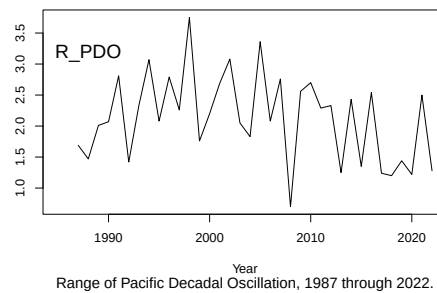
Figure 2(f): Range of Pacific Decadal Oscillation
