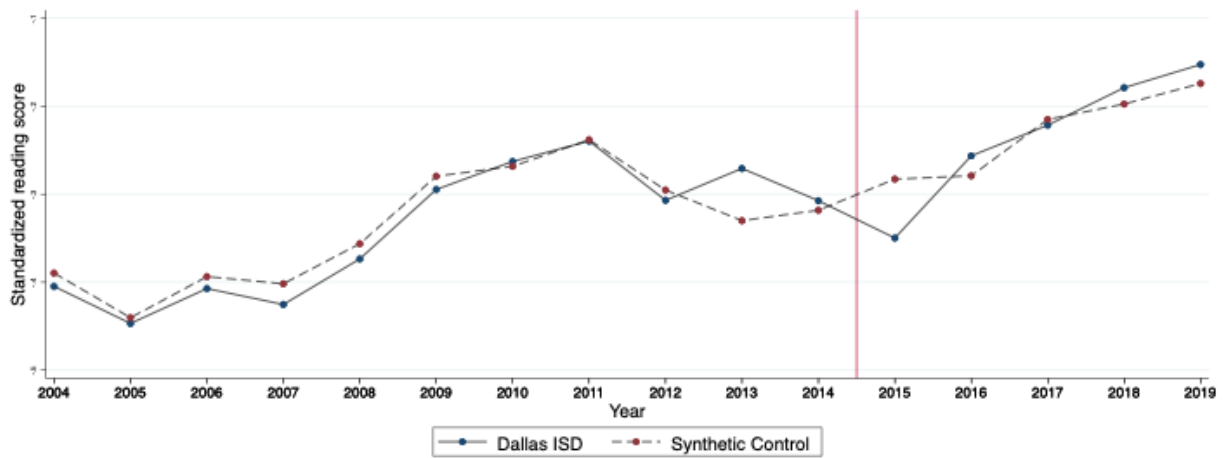
Figure 2. Synthetic control analysis of reading achievement.
