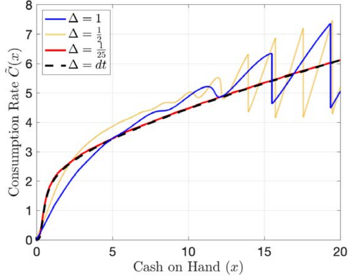
Figure 1: Consumption functions for a present-biased consumer ( \beta = 0.5 ) as \Delta \rightarrow 0 . The buffer stock consumption model is presented in Sections 2 and 3 below, and Section 4.2 provides calibration details.
