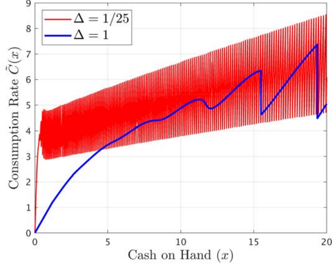
Figure 5: Consumption functions holding the \frac{\tilde{c}}{c} ratio constant ( \beta = 0.5 ).
