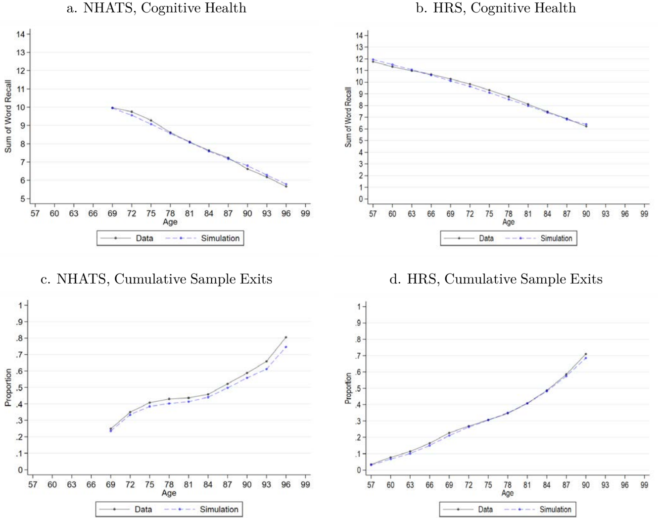
Figure 5: Model Fit
