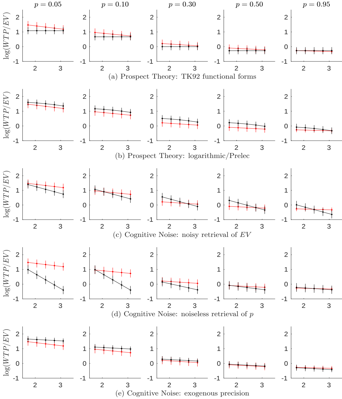
Figure 9: Predictions of alternative stochastic models of lottery valuation, using the same format as in Figures 7-8 (but only for selected values of p ). Each row shows the predictions of the baseline model (in red) and one alternative model (in black).
