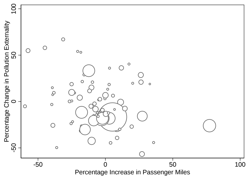
Figure 6B. The Effects of Total Passenger Miles on the Pollution Externality
