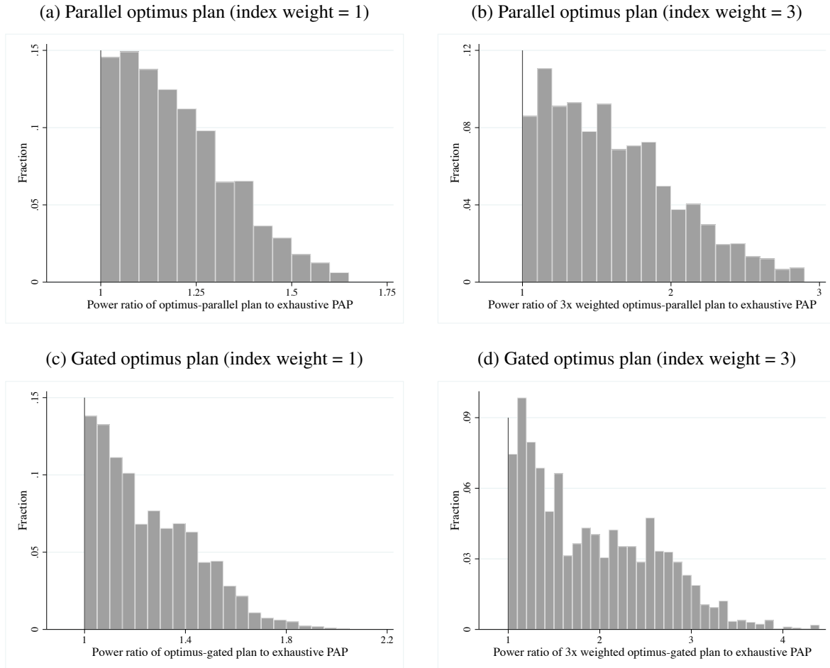
Figure 2: Distribution of Relative Power of Optimus Plans versus Exhaustive PAP
