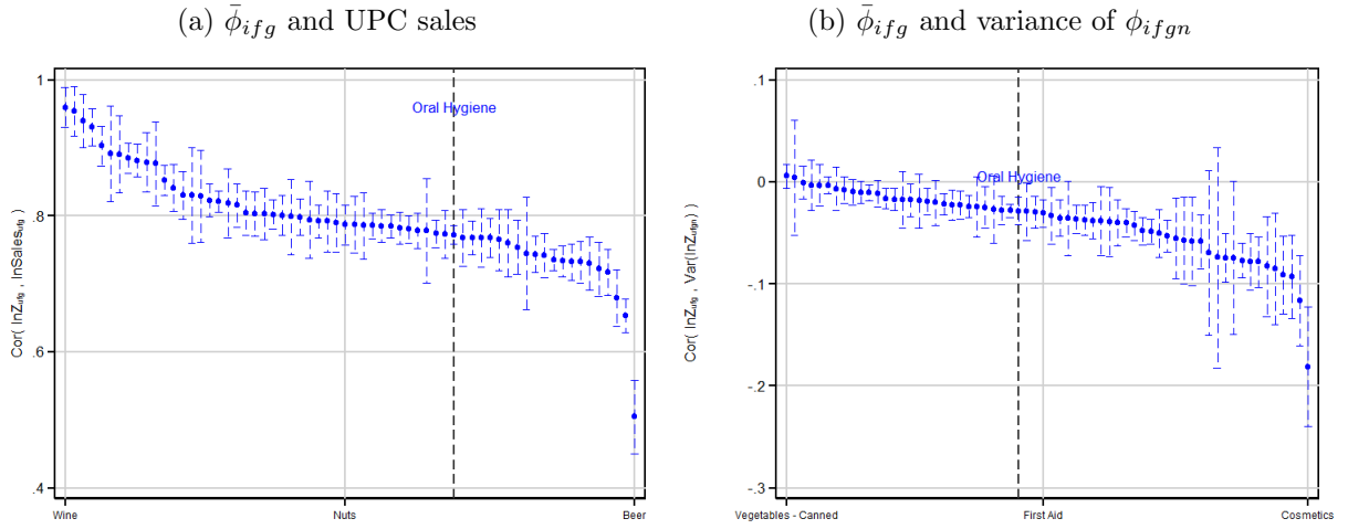
Figure A.3: Demand shifters and Segments (All UPC) - Type (Consumer Panel)
