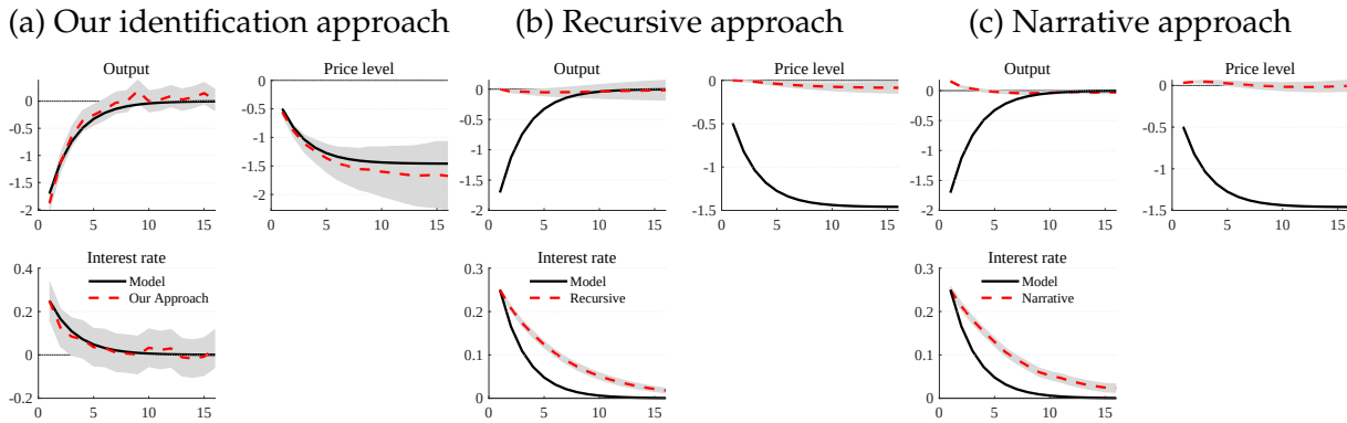
Figure 9: Comparison of identification approaches (baseline)
