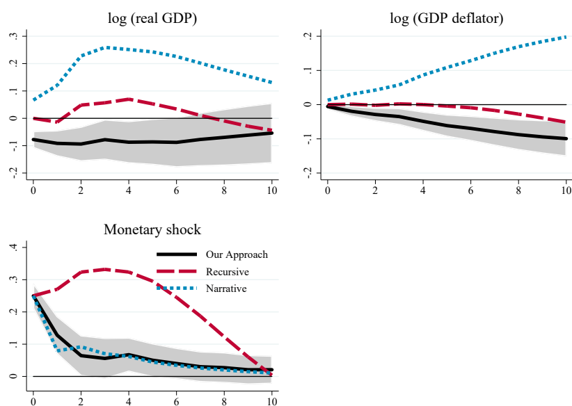
Figure 7: VAR results across identification approaches
