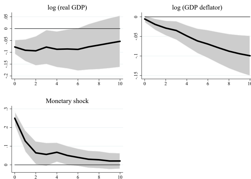
Figure 5: VAR results
