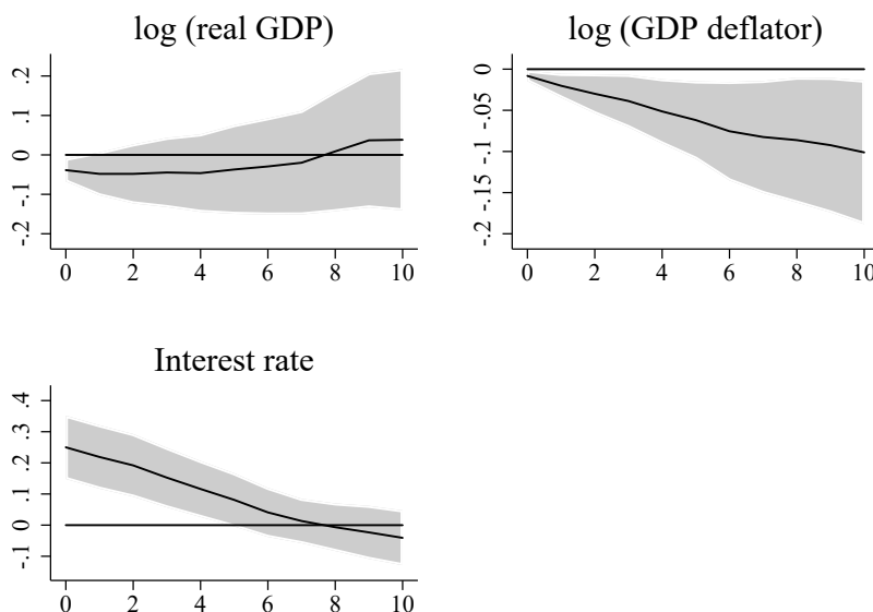
Figure 2: Local projections
