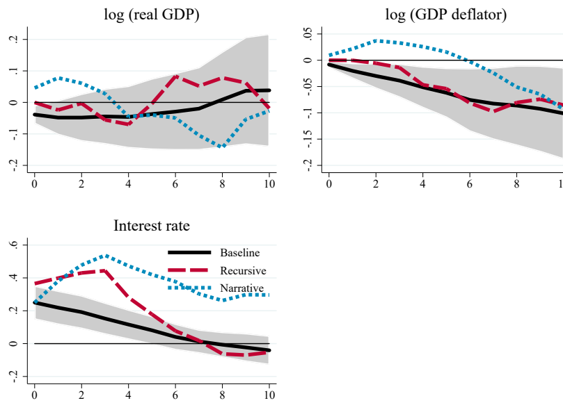
Figure 6: Local projection results across identification approaches
