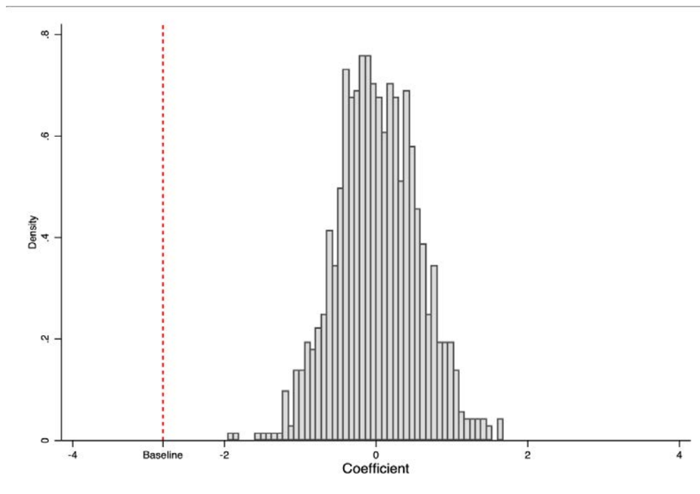
Figure 8: Randomization Inference
