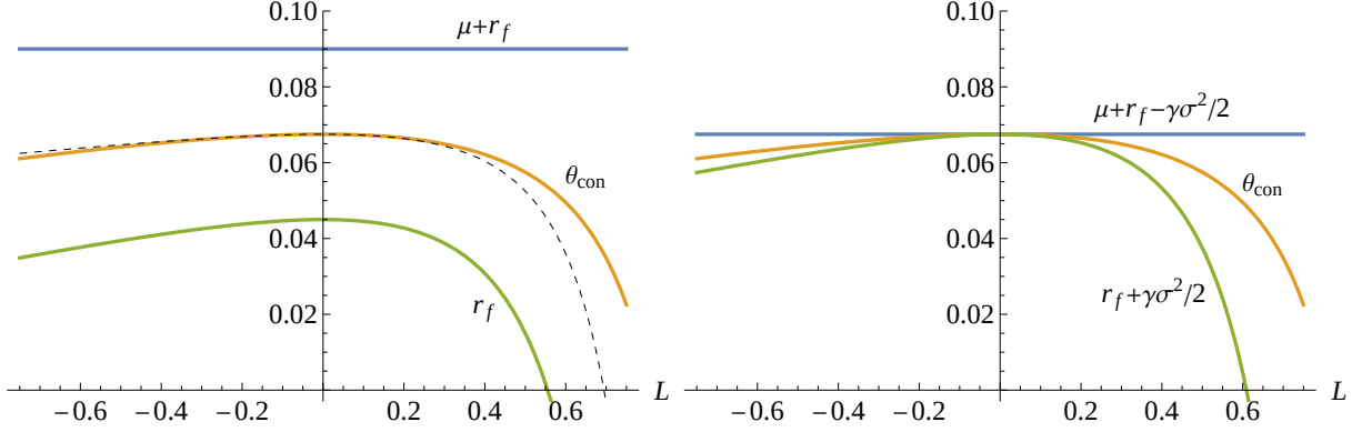
Figure 1: \theta_{\text{con}} and the upper and lower bounds for various deterministic jump sizes L , with \gamma = 2 , \sigma = 0.15 , \omega = 0.02 , \mu + r_f = 0.09 . Jumps are bad news if L is positive and good news if L is negative. The dashed line in the left panel indicates the midpoint of the riskless rate and expected return on the risky technology.
