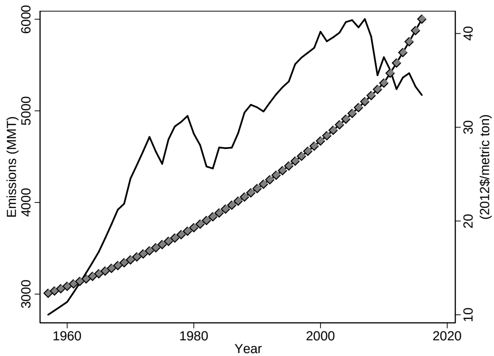
Figure A.5: U.S. Economy CO 2 Emissions and Social Cost of Carbon Estimates.
