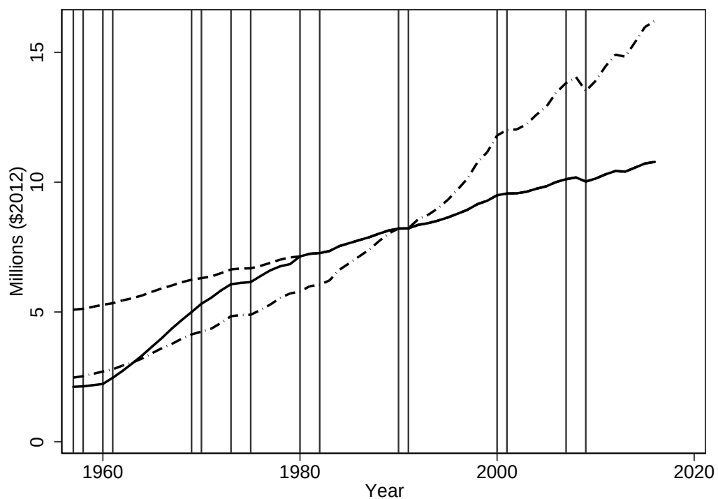
Figure A.4: VSL under various assumptions.
