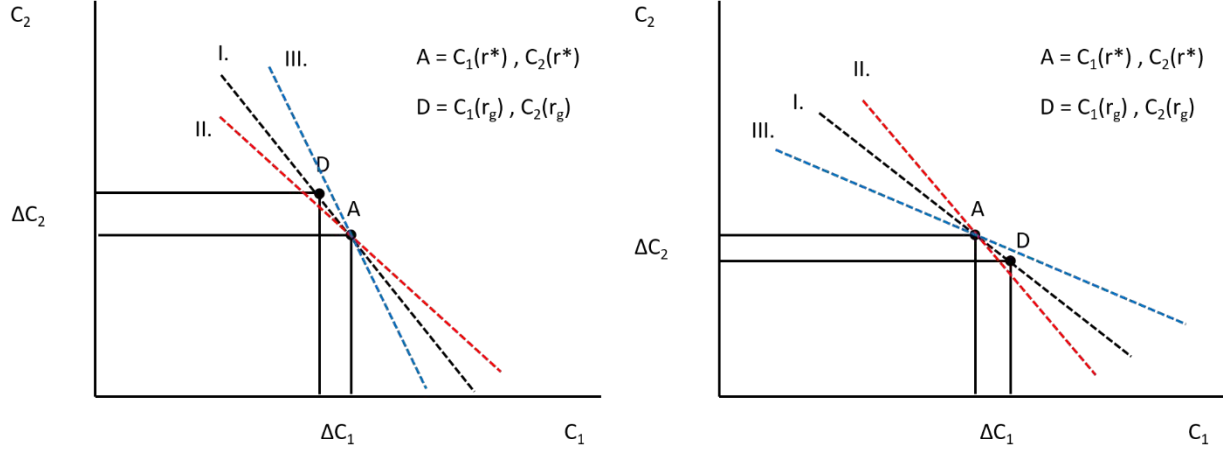
Figure A.1: Comparison of consumption, damage, and net consumption with r^* and r_g .
