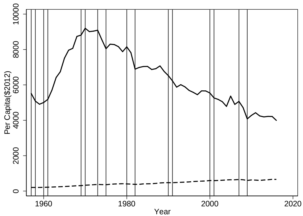
Figure A.6: Real, Per Capita Air Pollution and CO 2 GED.
