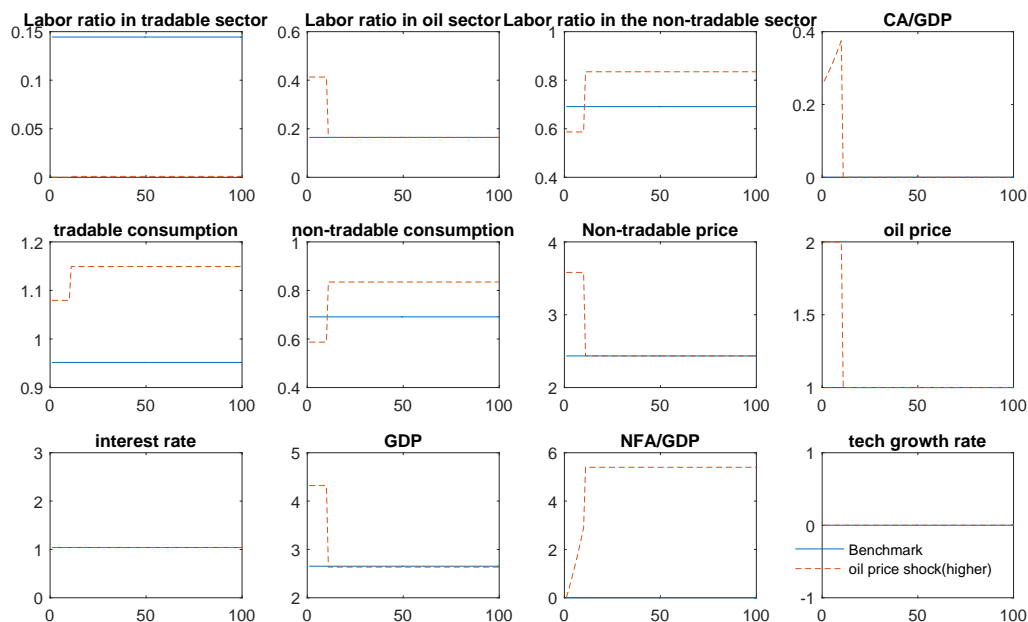
Figure 11: Case A, \alpha^N > \alpha^T
